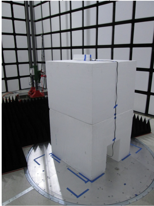
RADIATED BACK PHOTO (ABOVE 1 GHz)
