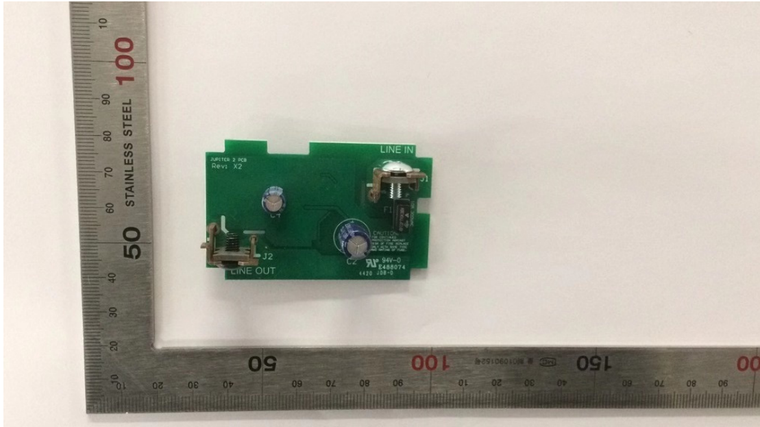
View of power supply board for CSC-SC-A-5B-UNV-WH
