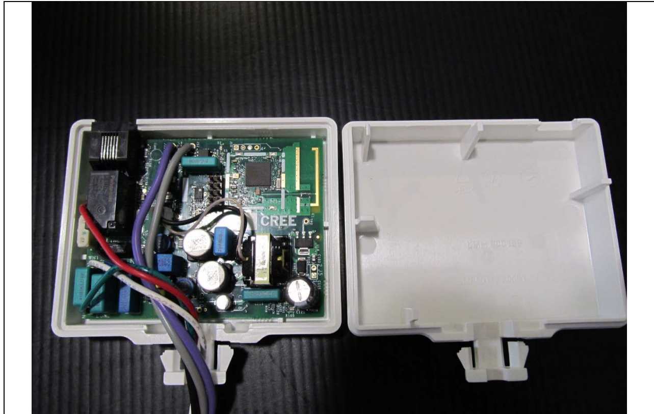
Top Side of Relay Board In Enclosure (CIF-10VC1-CWC-SNSR)
