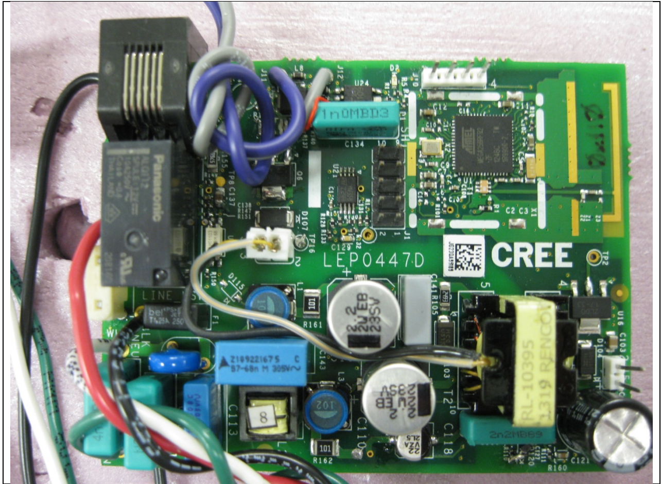
Top Side of Relay Board, Zoomed In (CIF-10V-CWC-SNSR)
