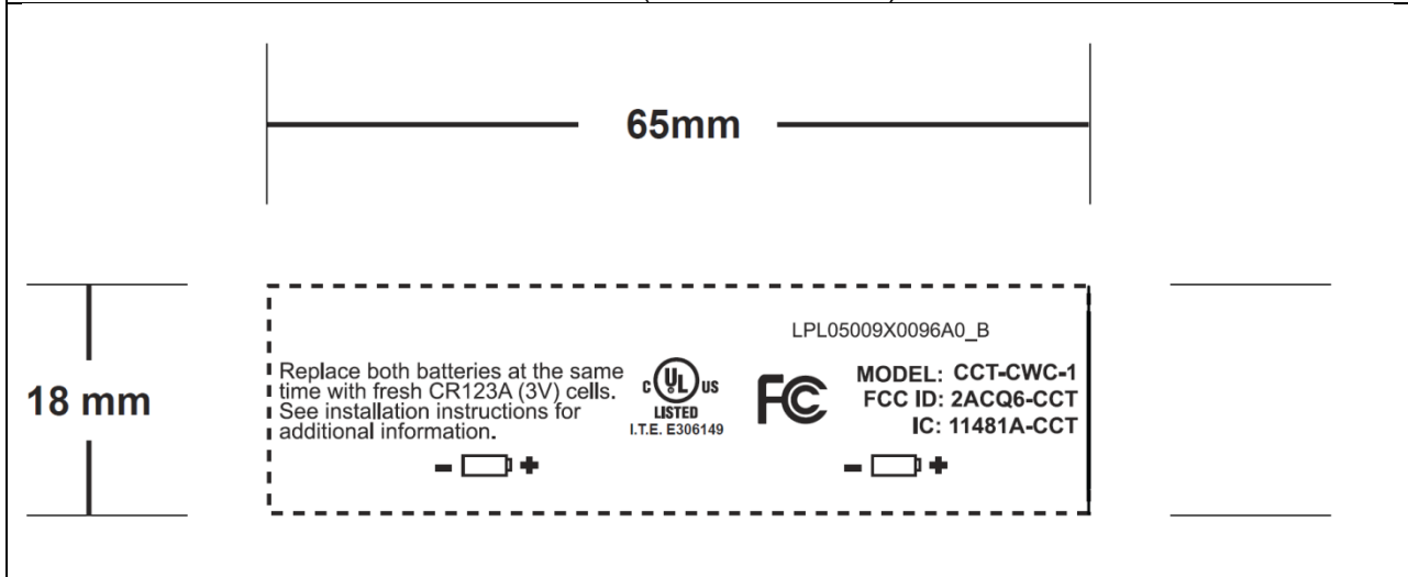
Label Drawing
