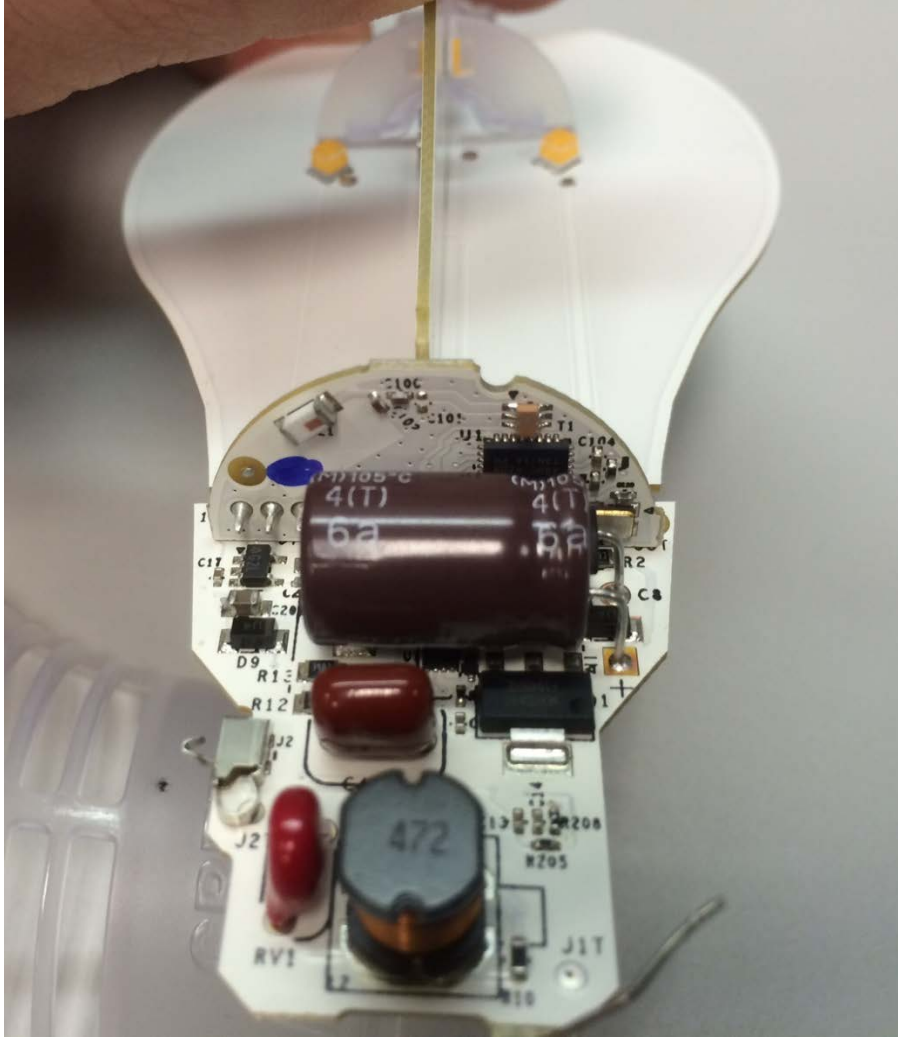
BA19 – Power Supply and RF Daughter Card (Bottom)
