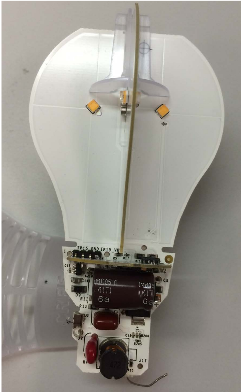
BA 19 – Top View
