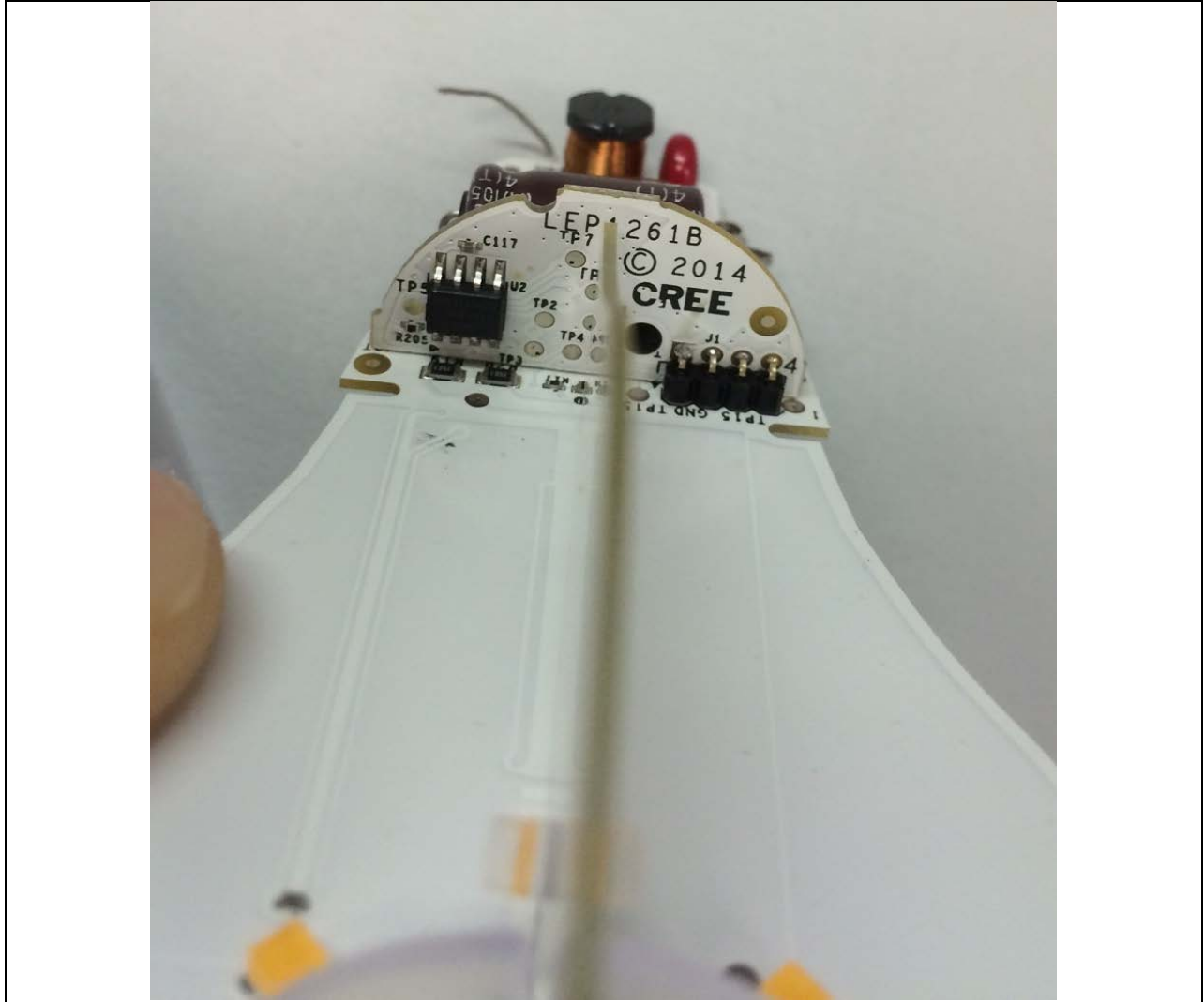
BA19 – RF Daughter Card (Top)
