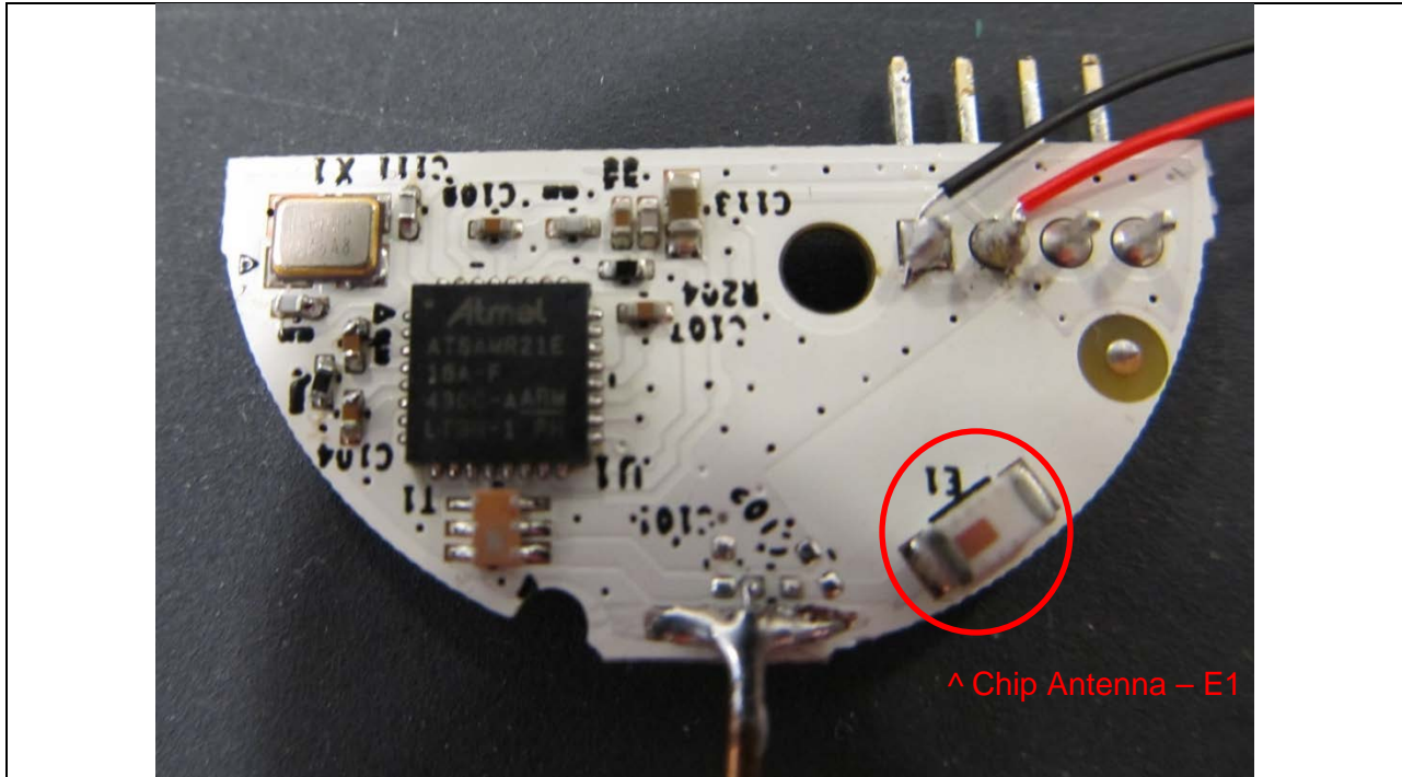
RF Daughter Board – Top
