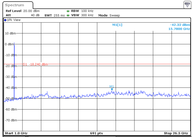
802.11b on channel 06
