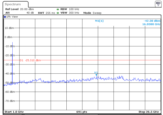
802.11g on channel 01
