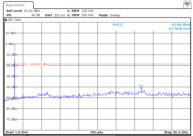
802.11b on channel 01
