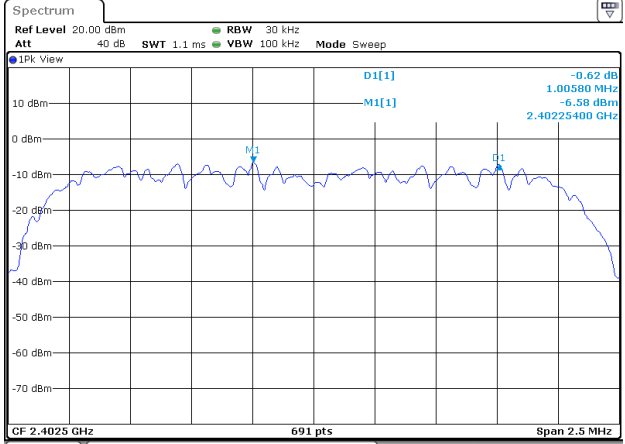
(2Mbps) Channel Separation plot on channel 00-01
