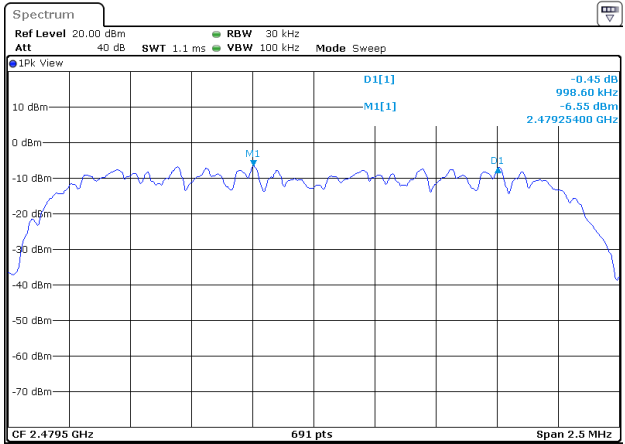
(2Mbps) Channel Separation plot on channel 77-78
