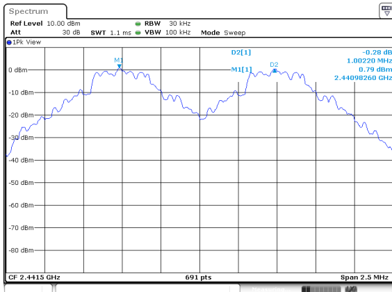
(1Mbps) Channel Separation plot on channel 39-40
