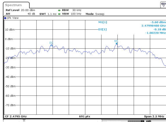
(2Mbps) Channel Separation plot on channel 77-78
