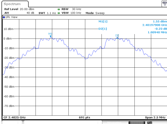
(1Mbps) Channel Separation plot on channel 00-01
