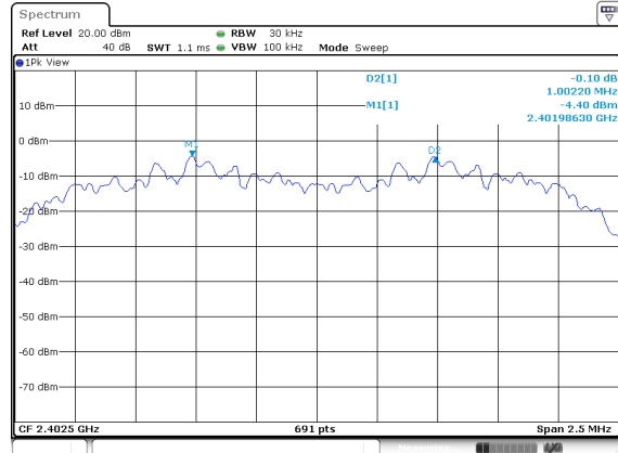
(2Mbps) Channel Separation plot on channel 00-01
