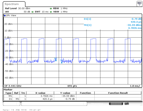
Package Transfer Time Plot CH39-2DH3
