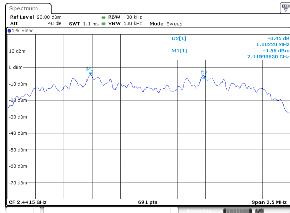
(2Mbps) Channel Separation plot on channel 39-40
