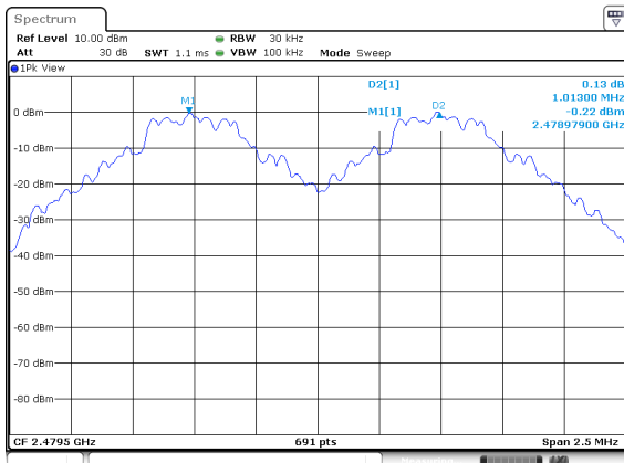
(1Mbps) Channel Separation plot on channel 77-78
