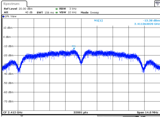
(802.11b) PSD plot on channel 1
