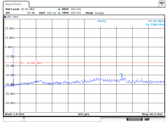
802.11b on channel 11
