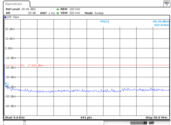
802.11 n20 on channel 11
