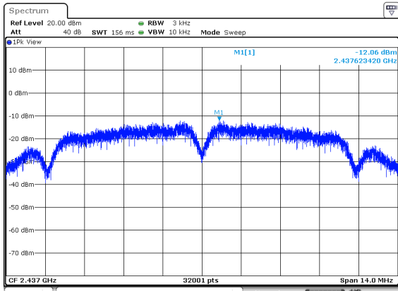
(802.11b) PSD plot on channel 6
