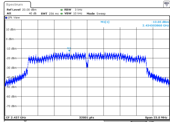
(802.11g) PSD plot on channel 6
