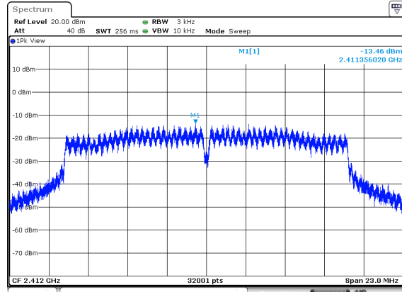
(802.11g) PSD plot on channel 1
