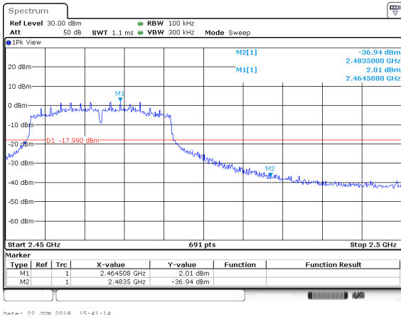
802.11n20: Band Edge-High Channel
