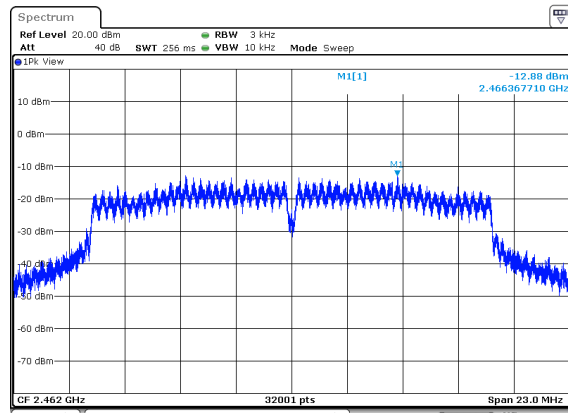
(802.11g) PSD plot on channel 11
