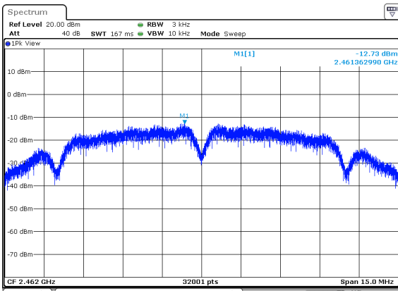
(802.11b) PSD plot on channel 11
