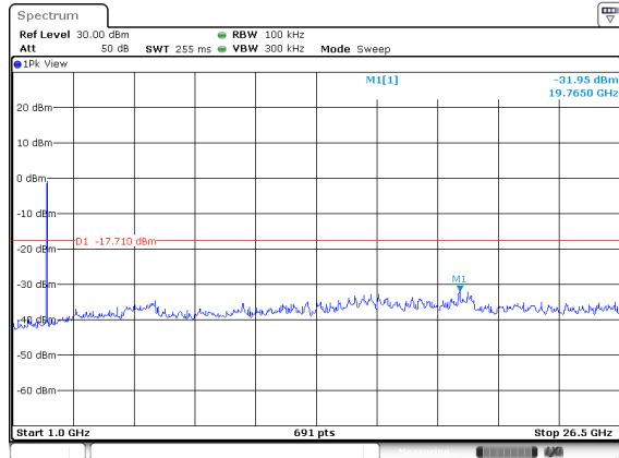
802.11g on channel 06
