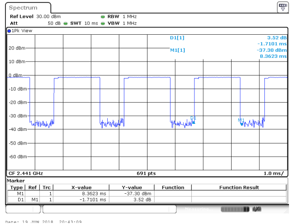
Package Transfer Time Plot CH39-2DH5
