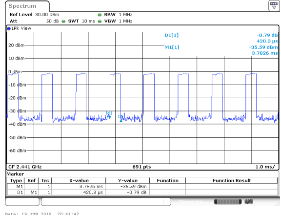
Package Transfer Time Plot CH39-2DH3
