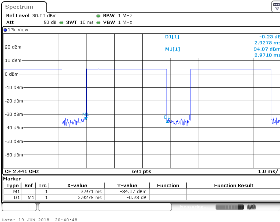
Package Transfer Time Plot CH39-DH5
