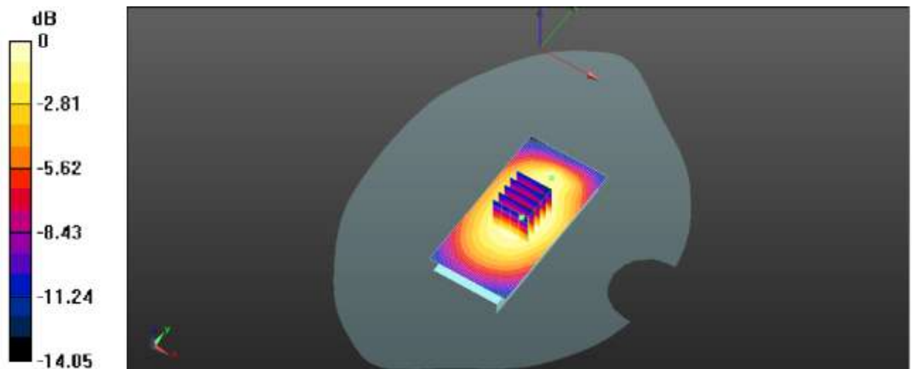
Plot 2: Body Rear Side (GSM850 Middle Channel)
