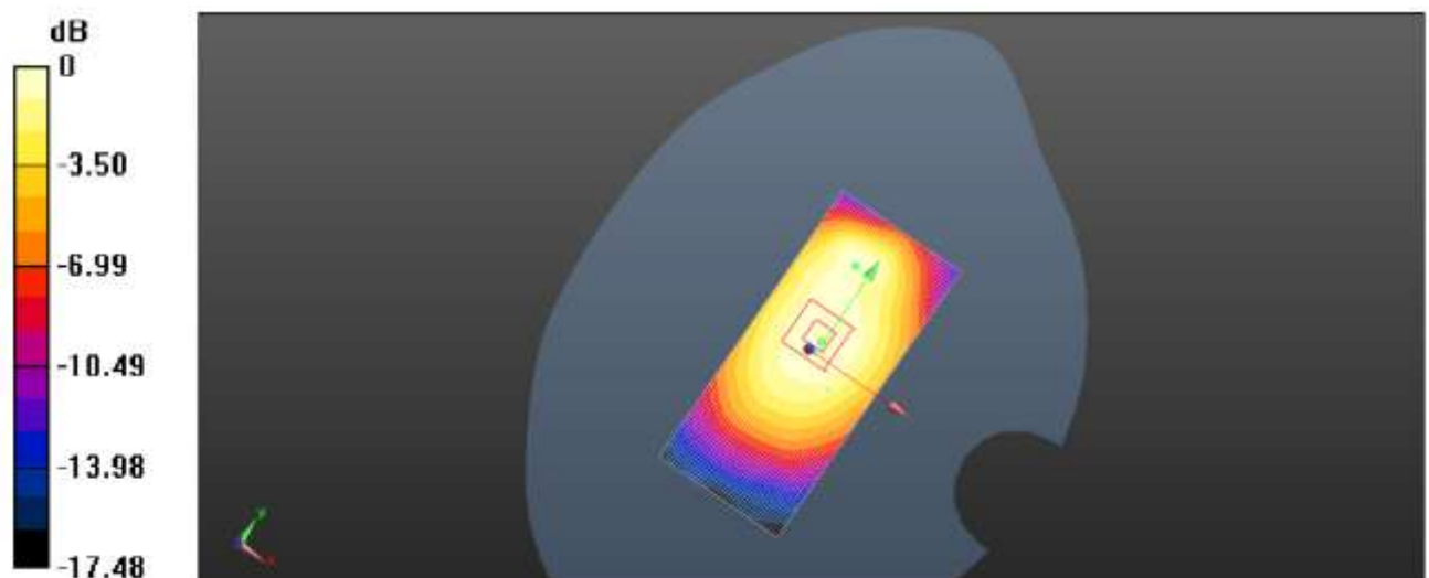
Plot 4: Body Rear Side (PCS1900 Middle Channel)
