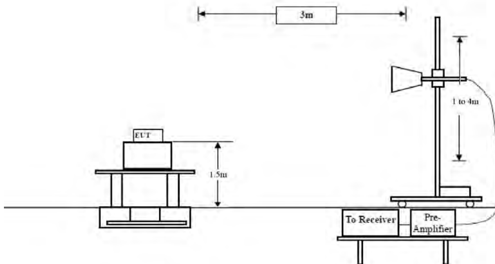
Figure 3. Above 1 GHz
