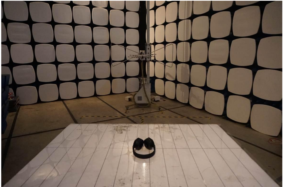
FCC RADIATED EMISSION TEST SETUP
