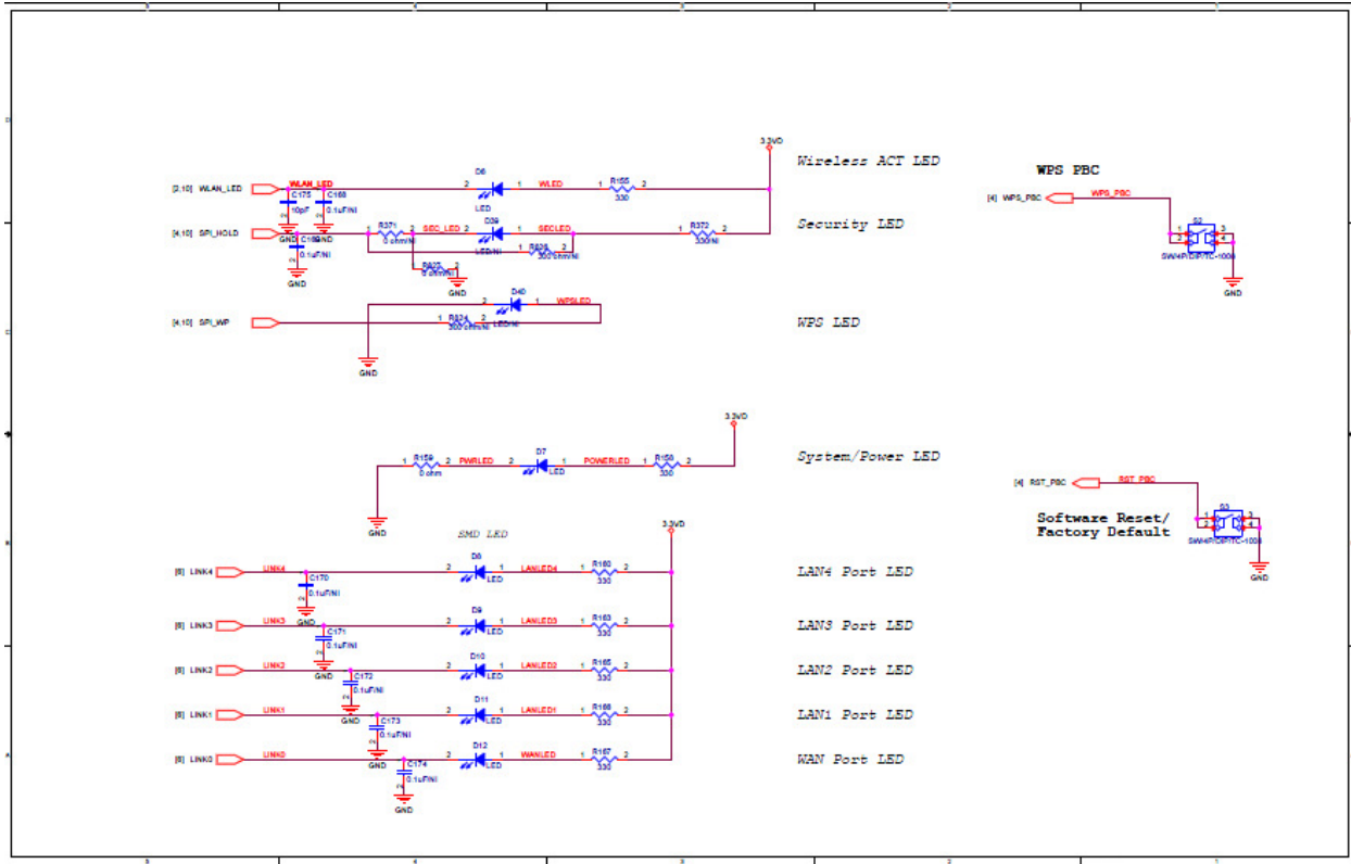
Figure 3: SKW75 Reference design schematic
