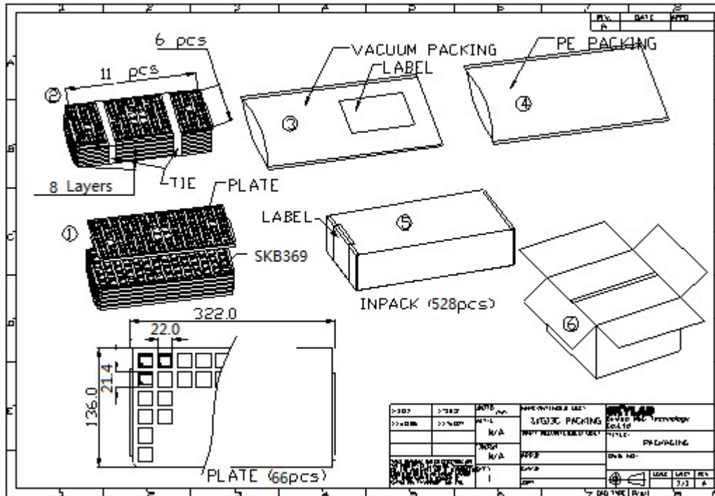
Figure 7: SKB369 Packaging
