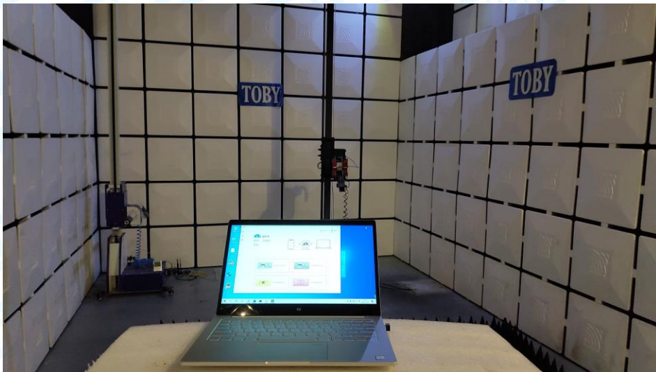
Photo of Setup for Radiated Emission (Below 1 GHz)
