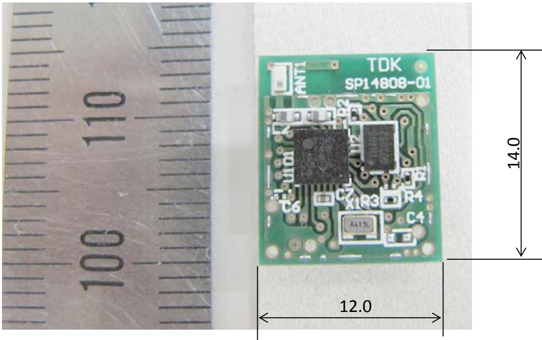
Top View
