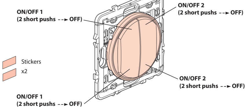
2-gang wireless and batteryless lighting control
