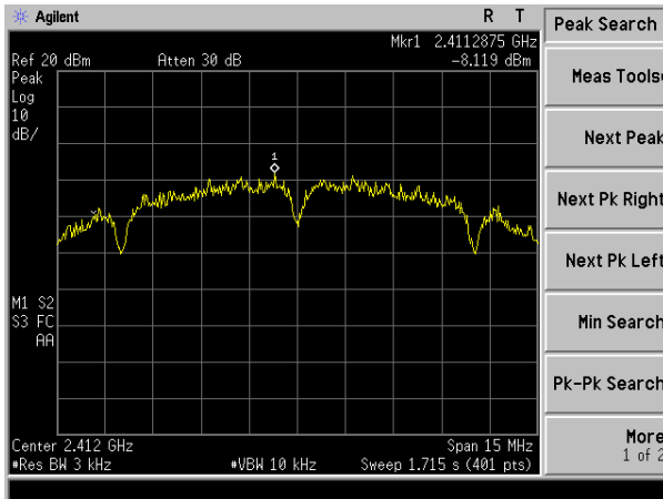
(802.11b) channel 1
