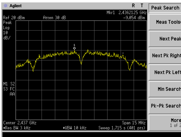
(802.11b) channel 6
