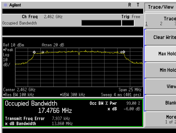
(802.11n20) channel 11
