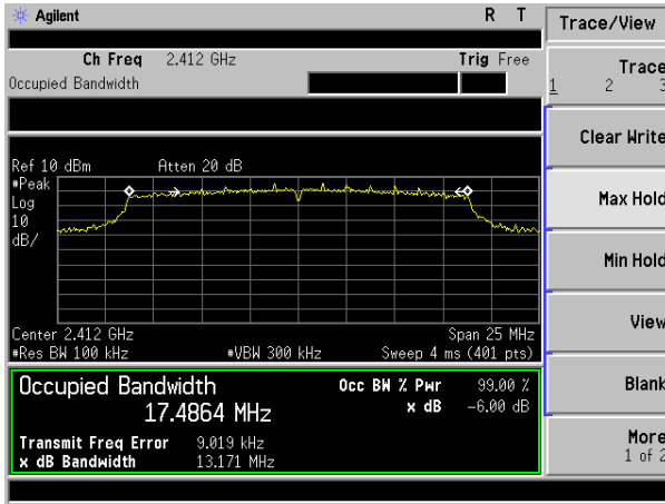
(802.11n20) channel 1
