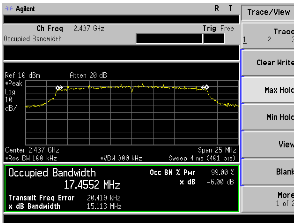
(802.11n20) channel 6
