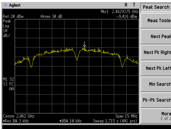
(802.11b) channel 11
