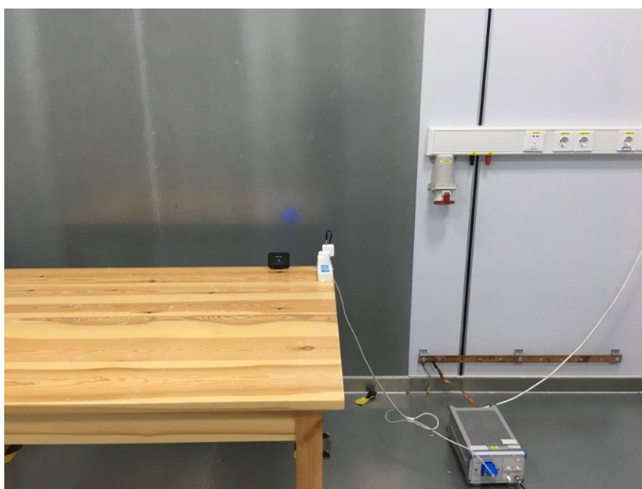
Power line conducted emission setup photo
