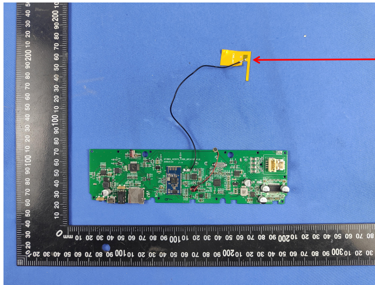
FPC ANTENNA
