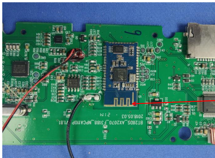
PCB antenna, not used
