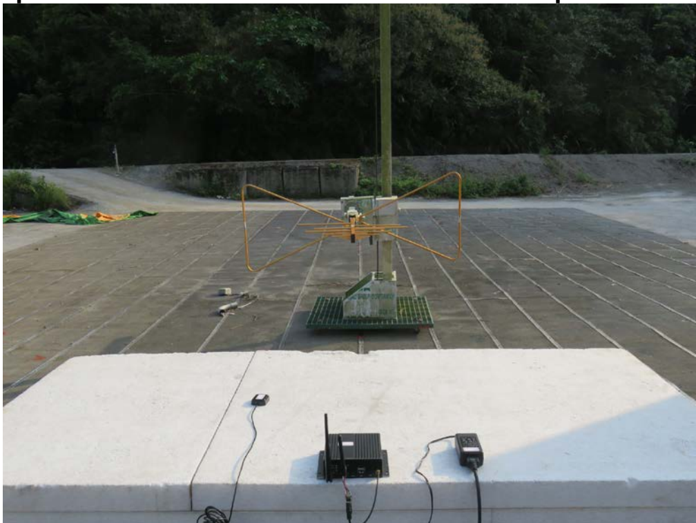
Photograph – Radiated Emission 1G Below Test Setup
