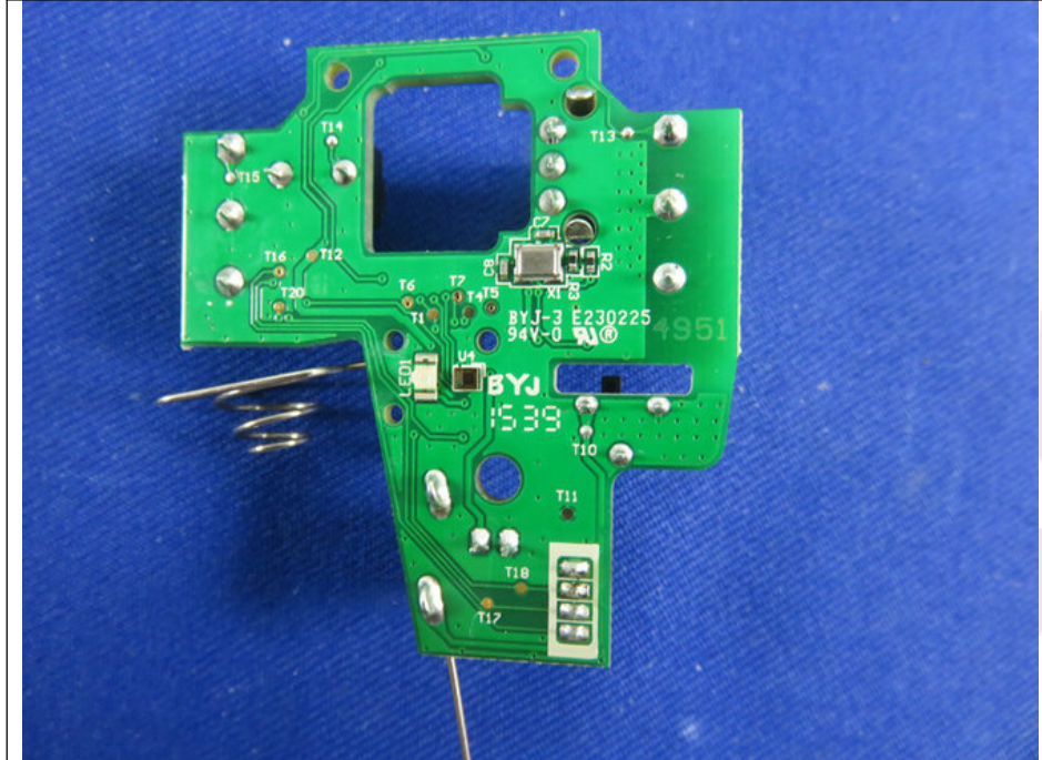
7. Figure PCB of the EUT-Back View
