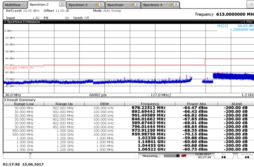
Figure 8.3-5: Conducted spurious emission of restricted band 30 MHz to 1.2 GHz, low channel
