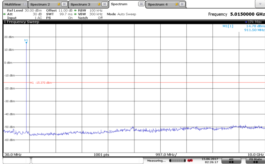
Figure 8.3-3: Conducted spurious emissions outside restricted band, Low channel
