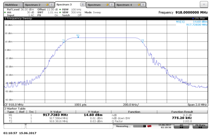
Figure 8.1-2: 6 dB bandwidth on high channel
