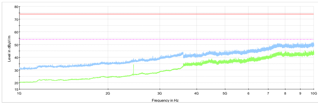
Figure 8.3-15: Cabinet Radiated spurious emissions 1 to 10 GHz, Receiver mode
