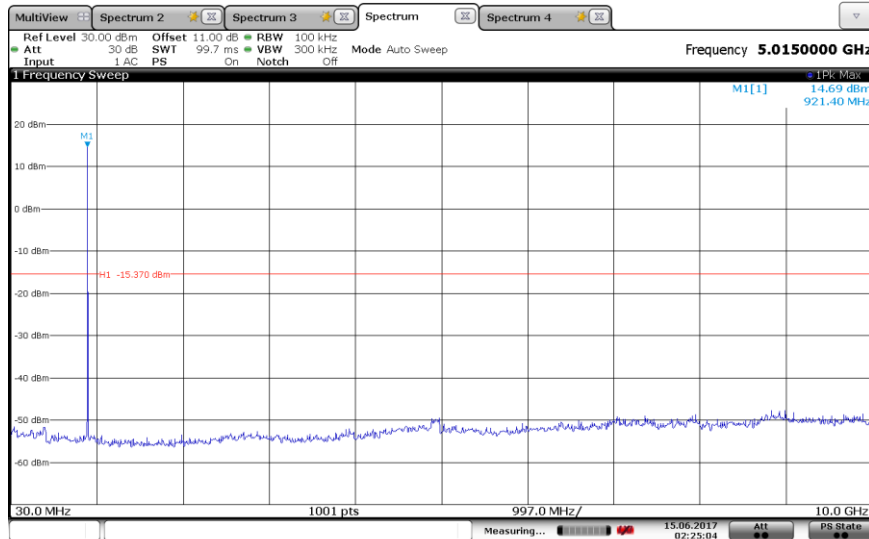
Figure 8.3-4: Conducted spurious emissions outside restricted band, High channel
