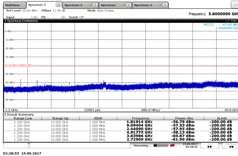
Figure 8.3-7: Conducted spurious emission of restricted band 1.2 GHz to 10 GHz, low channel
