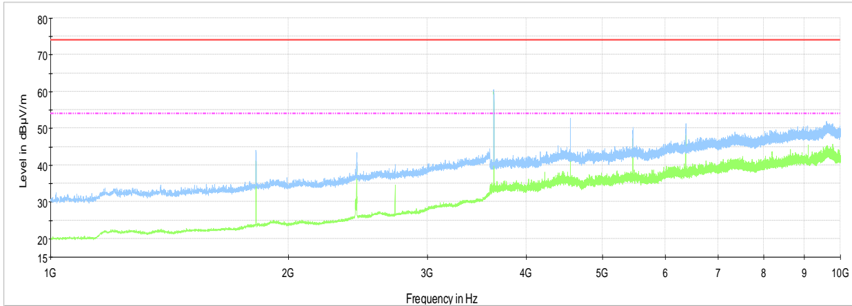
Figure 8.3-11: Cabinet Radiated spurious emissions 1 to 10 GHz, Low channel
