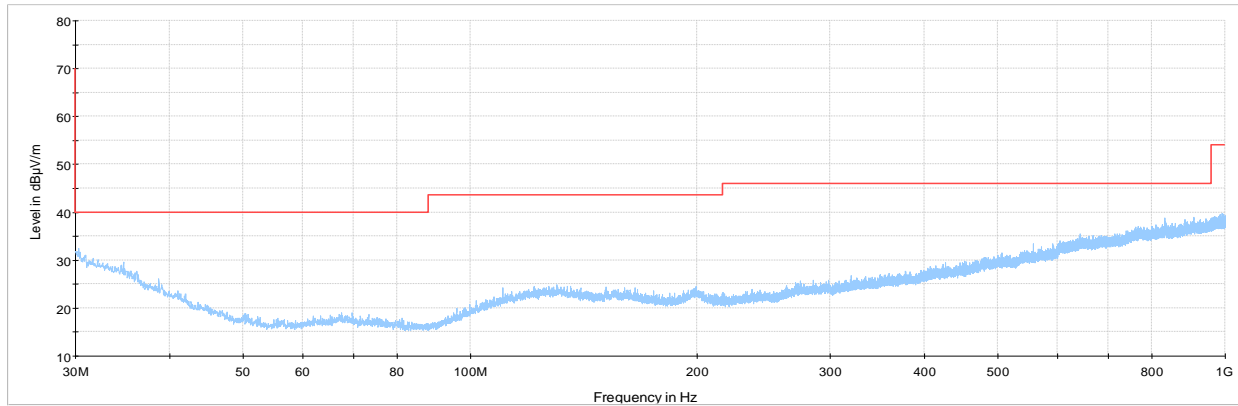
Figure 8.3-14: Cabinet Radiated spurious emissions 30 MHz to 1 GHz, Receiver mode
