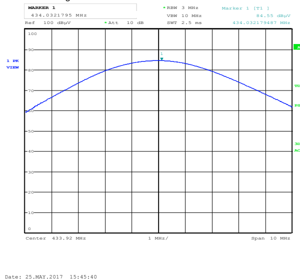
Figure 8.2-2: Field Strength of Fundamental plot
