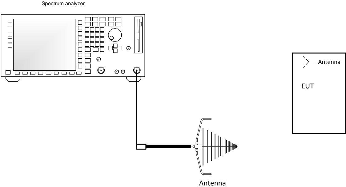
Figure 3.6-1: Setup diagram
