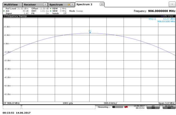
Figure 8.2-2: Output power on high channel
