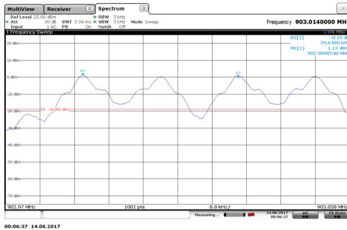
Figure 8.1-3: Carrier frequency separation
