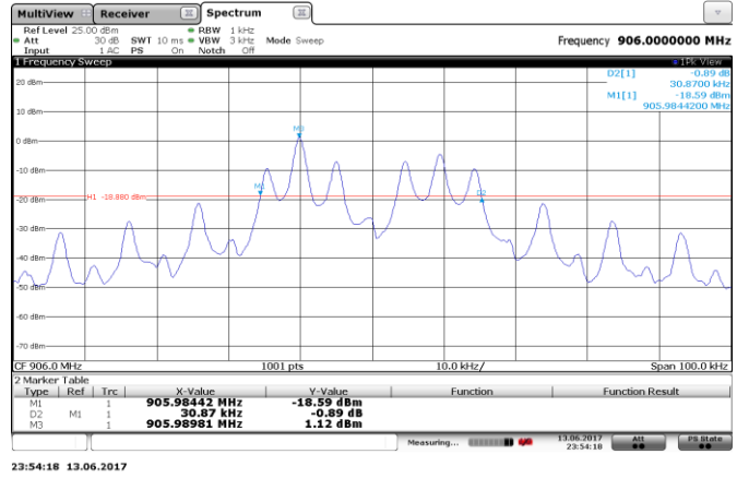
Figure 8.1-2: 20 dB bandwidth on hi channel
