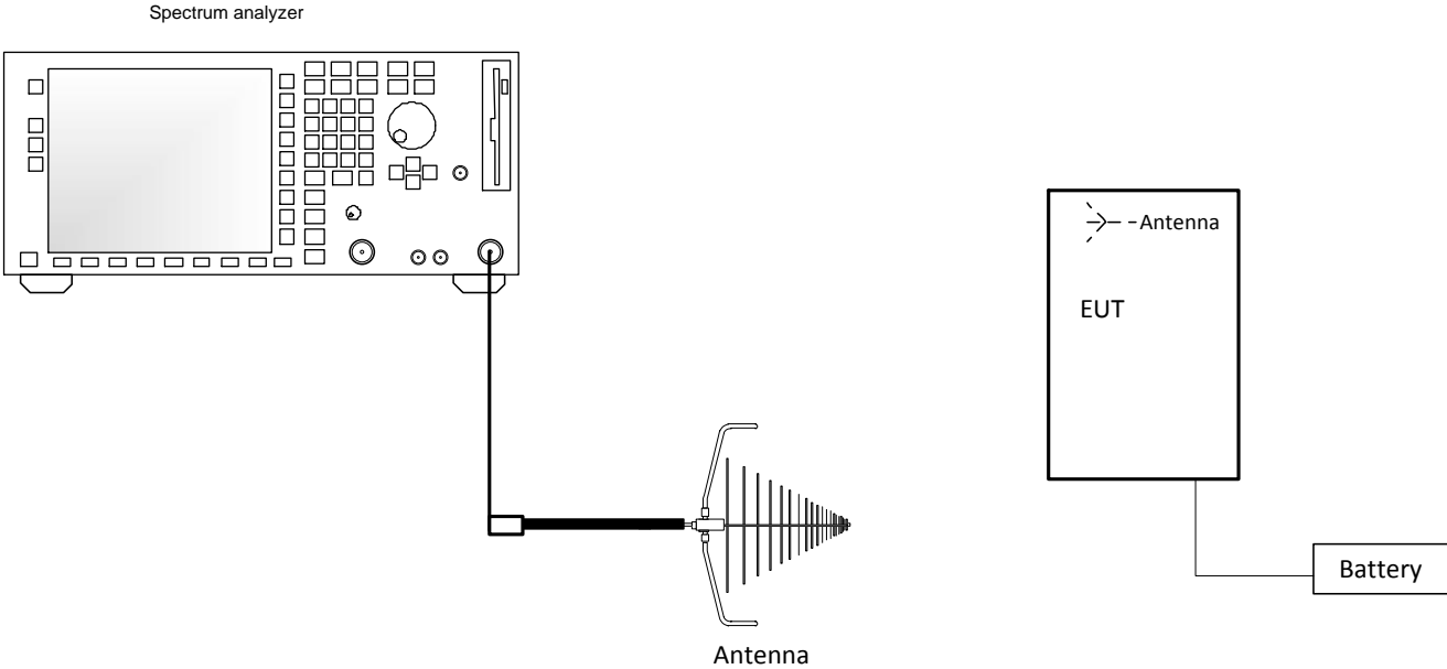
Figure 3.6-1: Setup diagram
