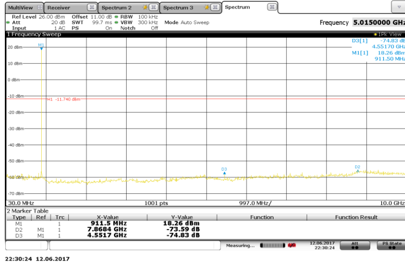
Figure 8.3-3: Conducted spurious emissions outside restricted band, Low channel
