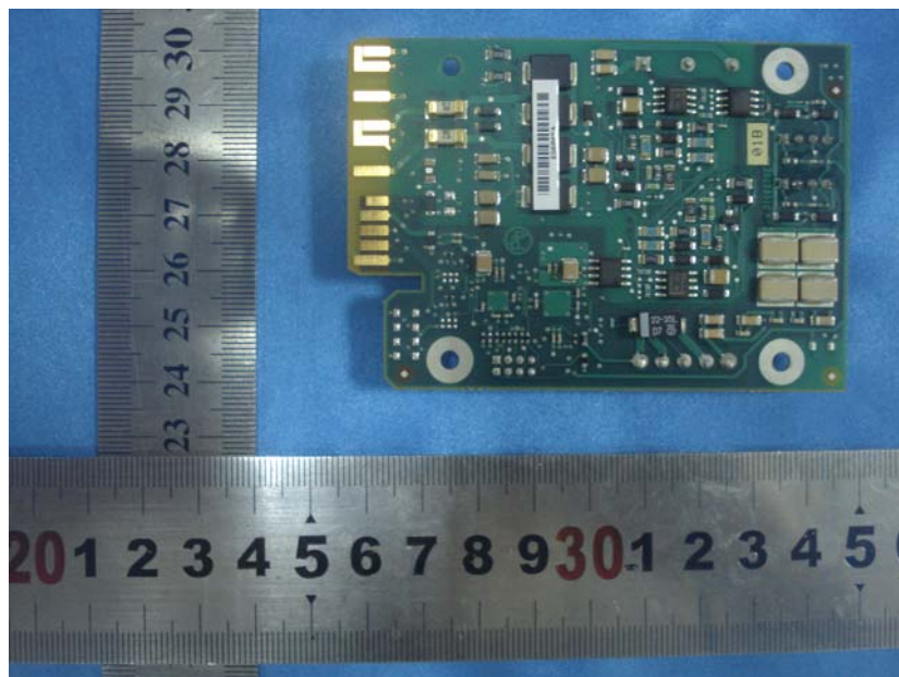
EUT – Circuit Board 2 Bottom View
