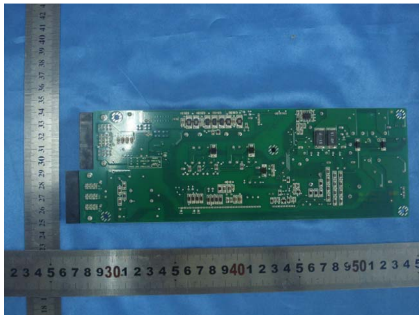
EUT – Power Supply MB Bottom View
