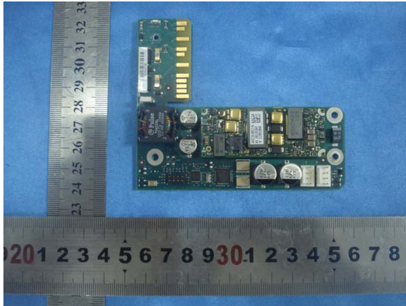
EUT – Circuit Board 1 Top View
