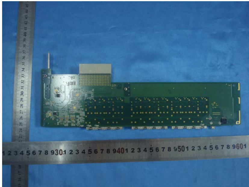
EUT – Circuit Board 3 Bottom View
