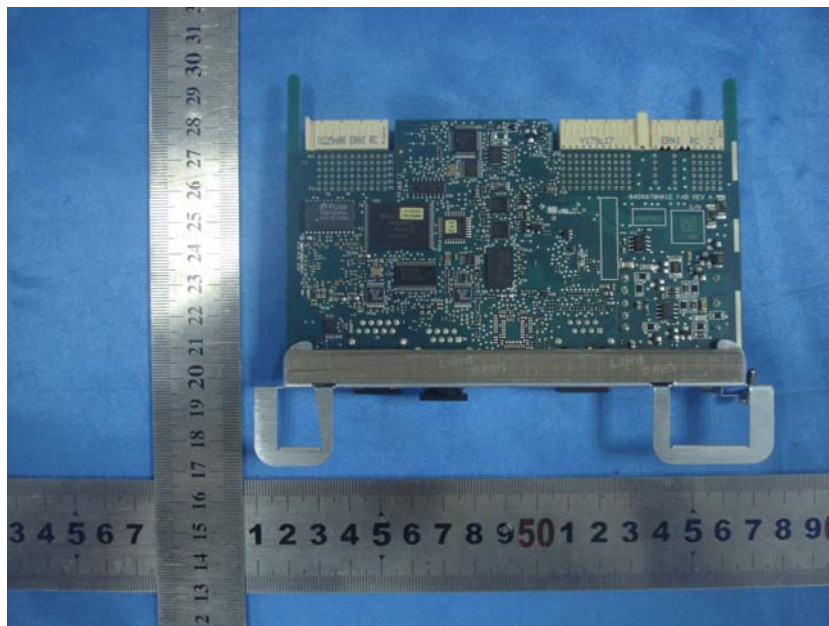
EUT – Circuit Board 4 Bottom View
