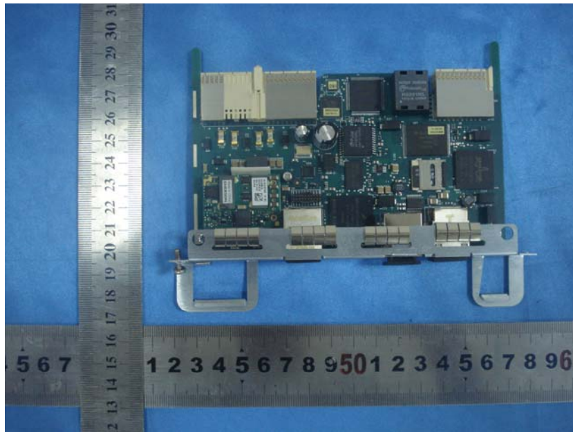
EUT – Circuit Board 4 Top View
