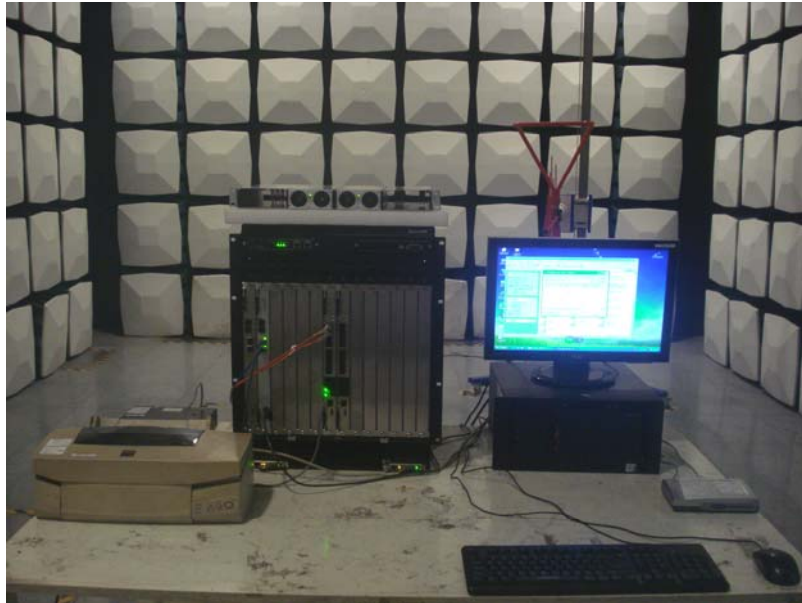
Radiated Emission Test Setup (Below 1GHz) Front View
