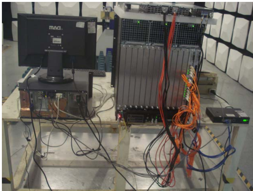
Radiated Disturbance Test Setup (Above 1GHz) Rear View
