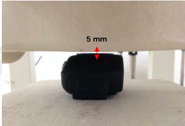
Fig.3 Front side to flat phantom
