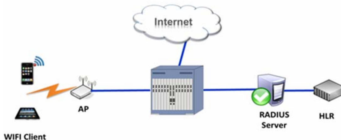
Figure 9-1 EAP-SIM authentication
