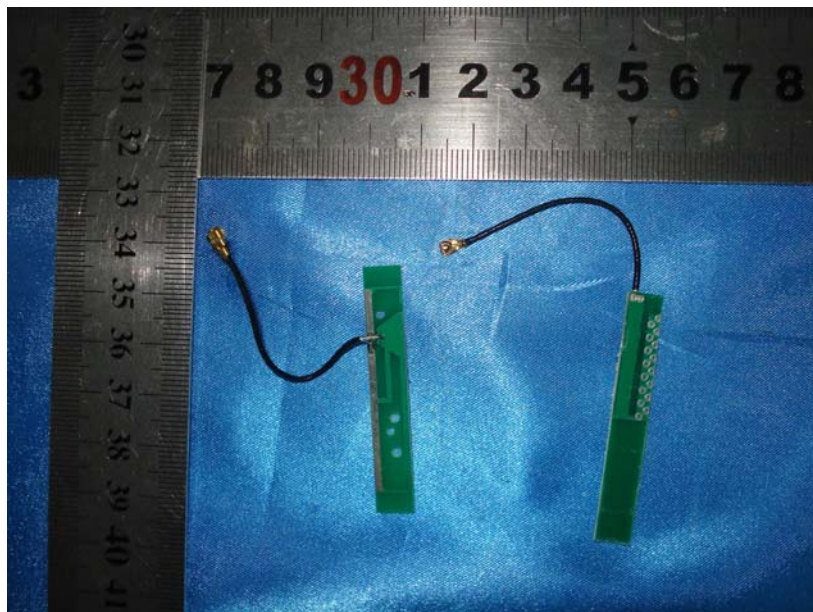
Antenna View
