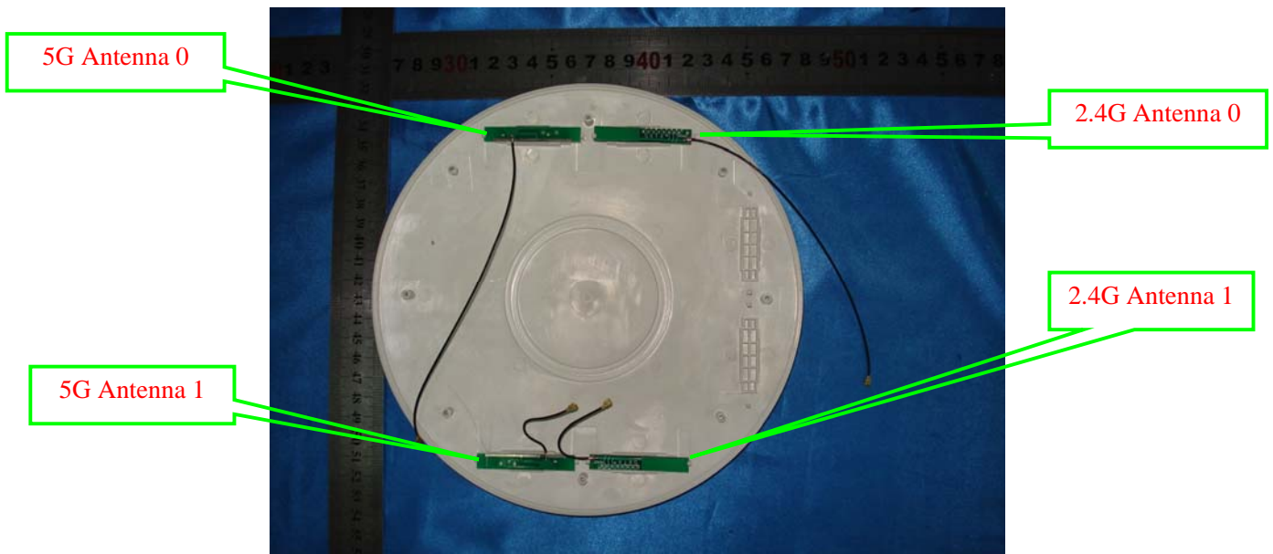
EUT – Cover off 2 View
