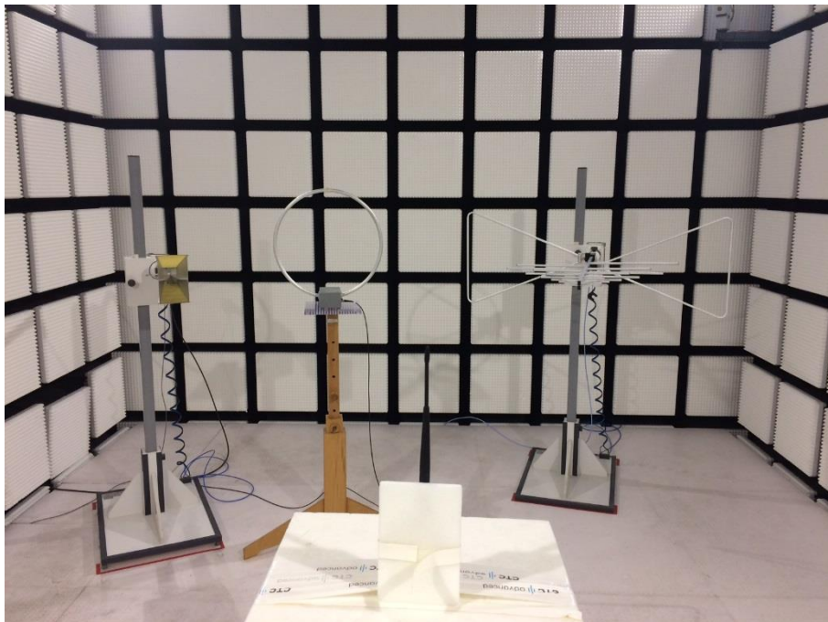
Photo 6: Chamber A – Spurious Emissions radiated 1GHz – 10 GHz
