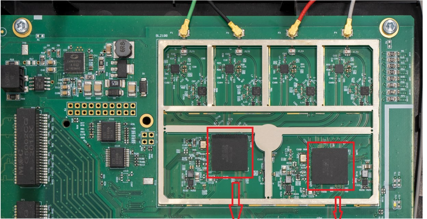
Broadcom BCM43684
