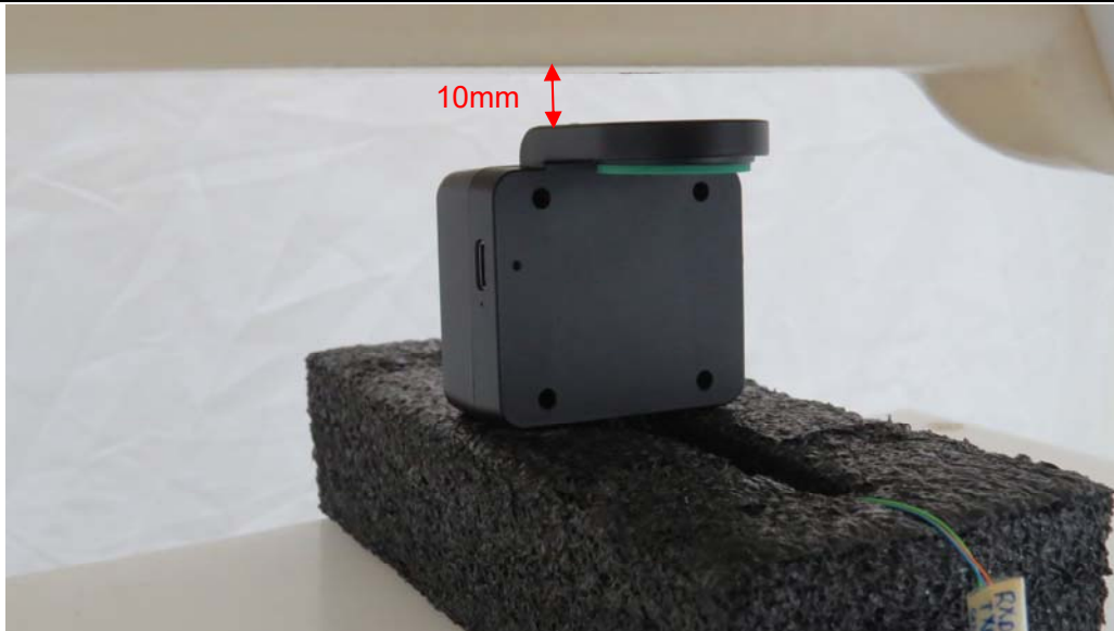
Picture 5: Top Edge, the distance from handset to the bottom of the Phantom is 10mm
