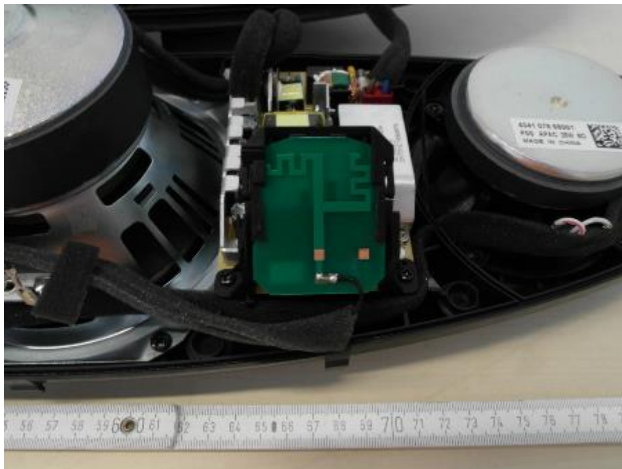
Photo 5: Transmit antenna
