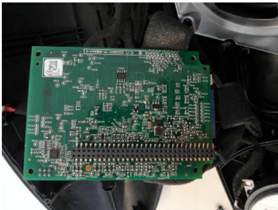
Photo 13: PCB 3 backside
