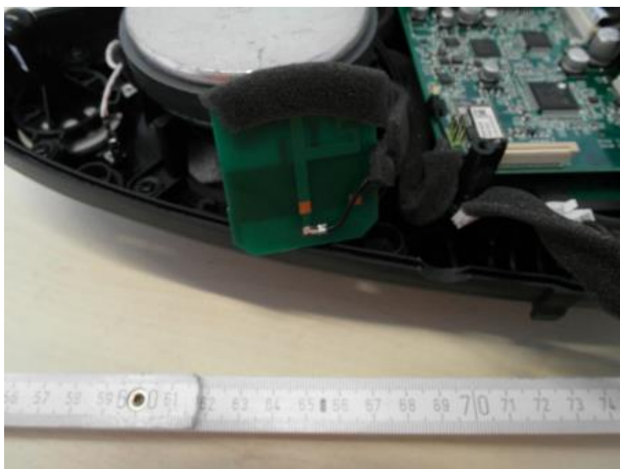
Photo 10: Antenna 2
