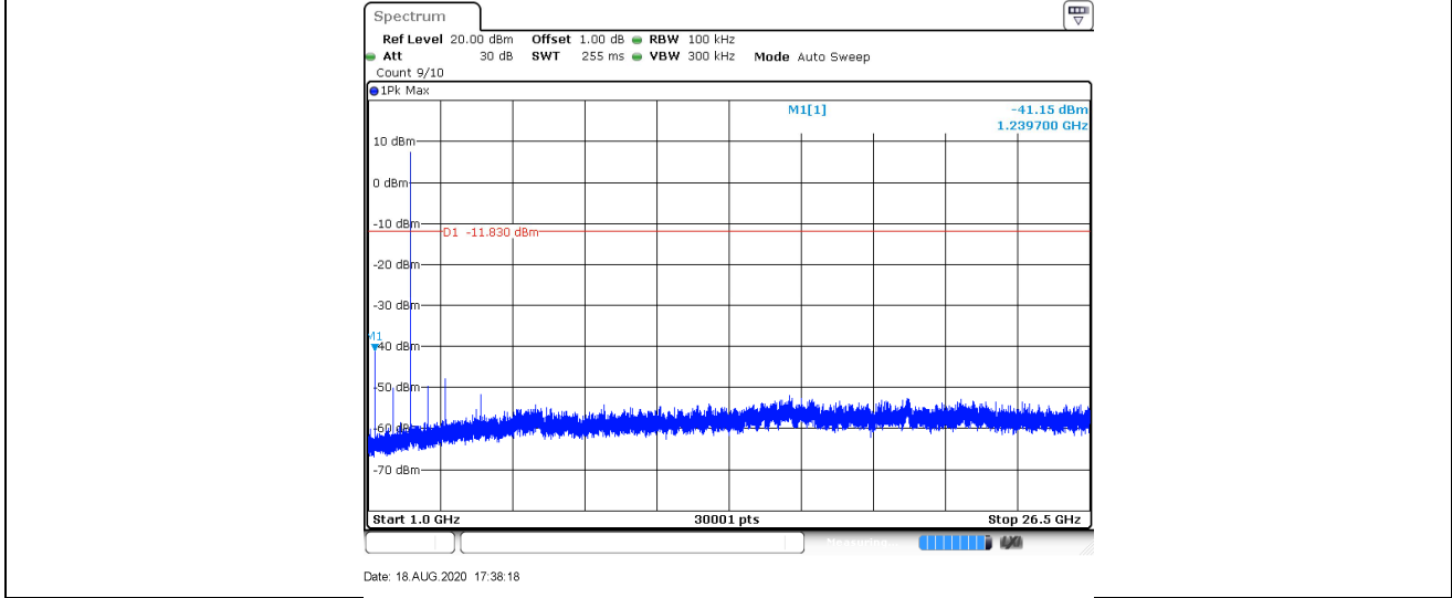
2DH5_Ant1_2402_0-Reference
