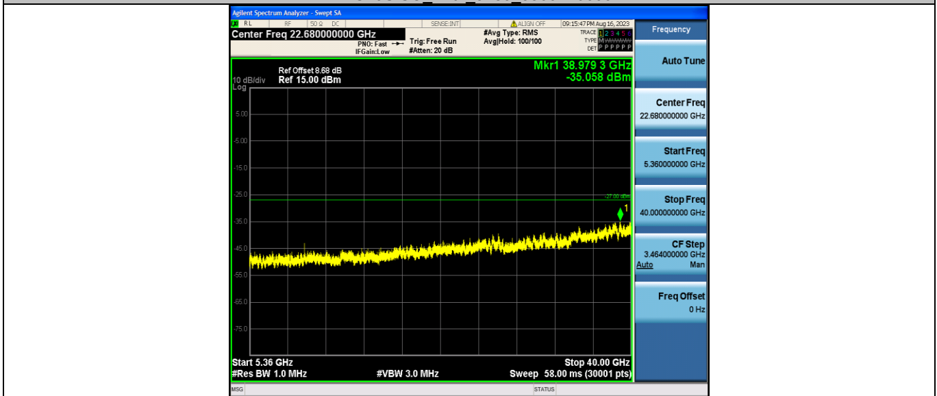
11AC20SISO_Ant1_5200_5360~40000
