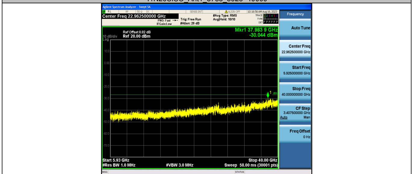
11N20SISO_Ant2_5785_30~5650
