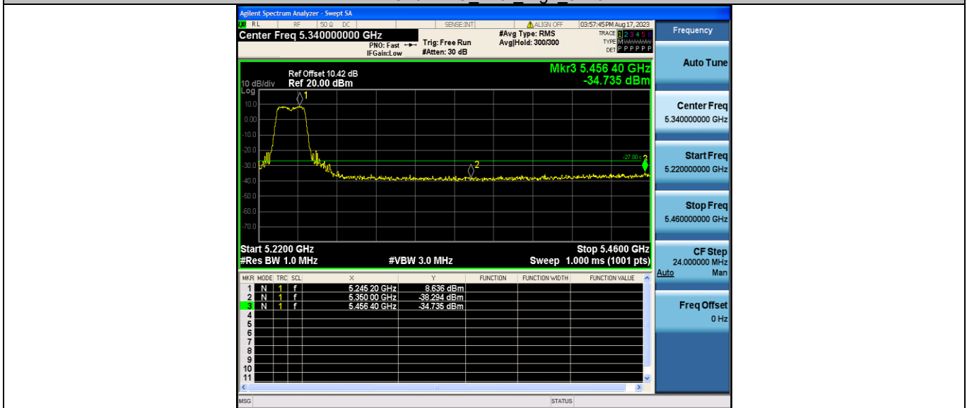
11AC20MIMO_Ant2_High_5240
