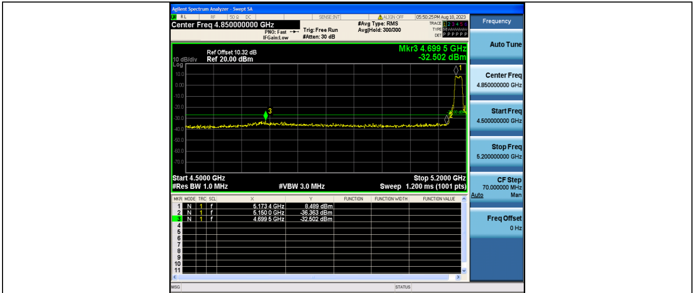
11AC20SISO_Ant2_Low_5180
