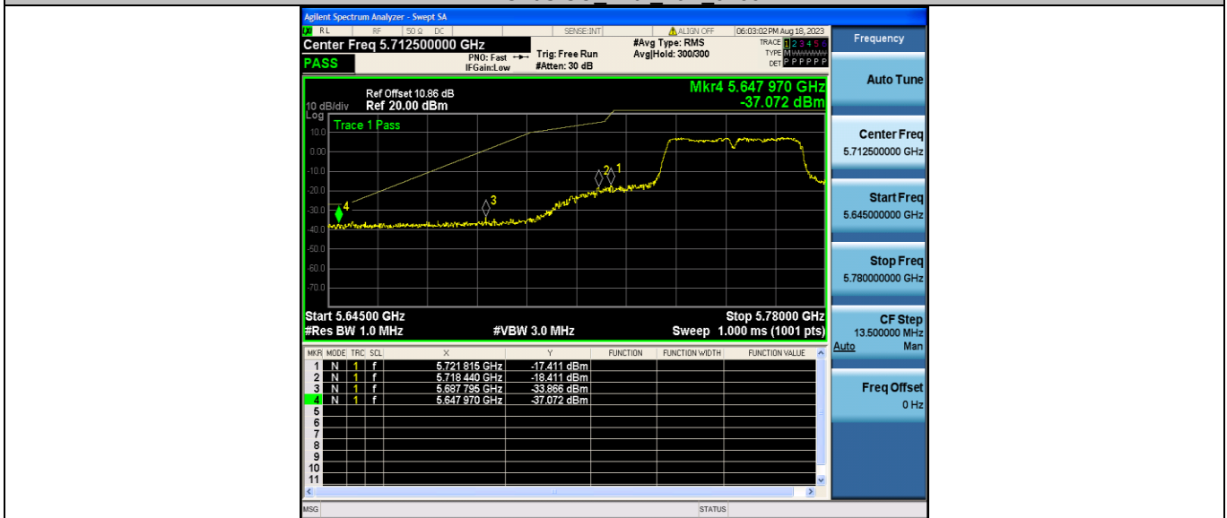
11AC40SISO_Ant2_Low_5755
