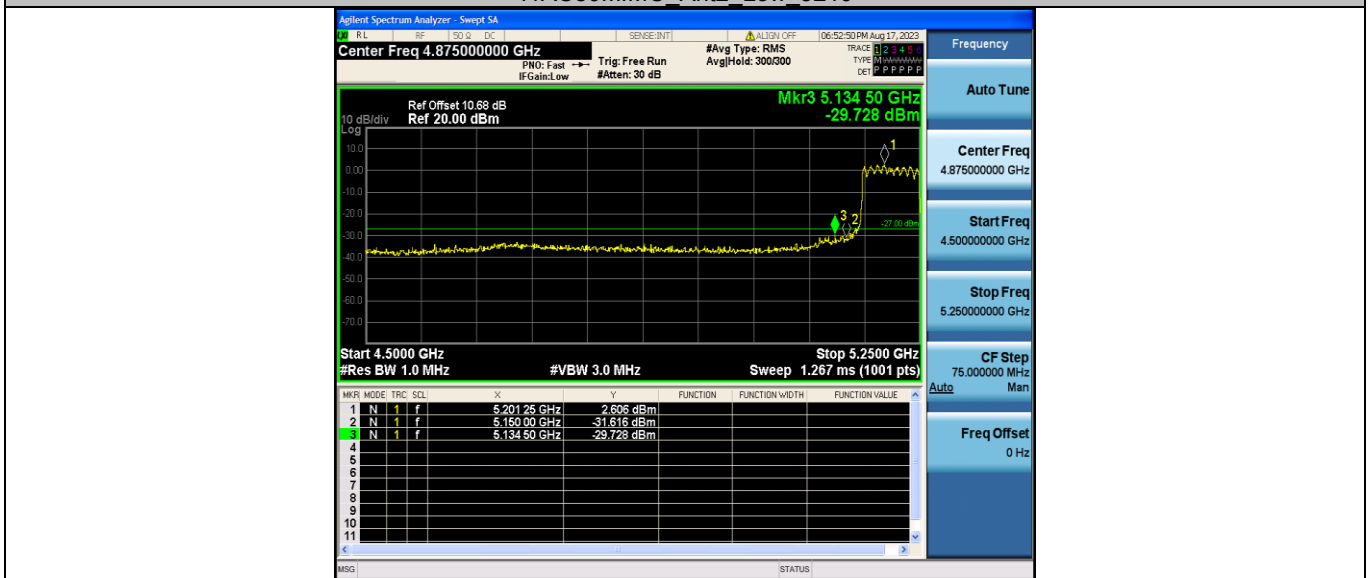
11AC80MIMO_Ant1_High_5210
