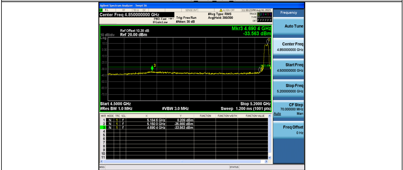
11N20MIMO Ant1 High 5240
