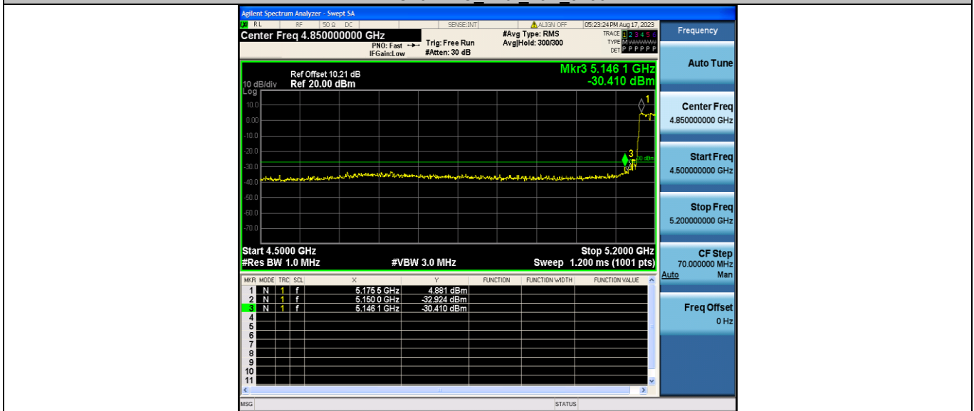
11AC40MIMO_Ant1_High_5230
