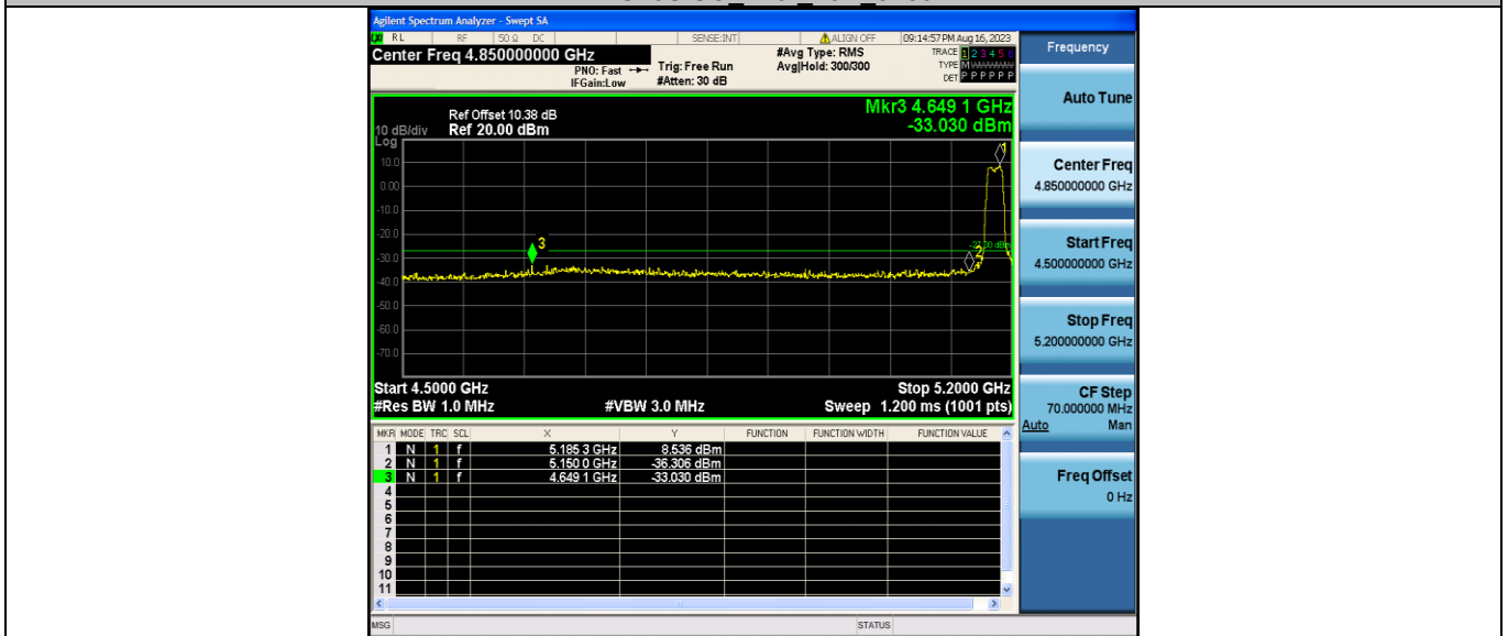
11AC20SISO_Ant1_High_5240
