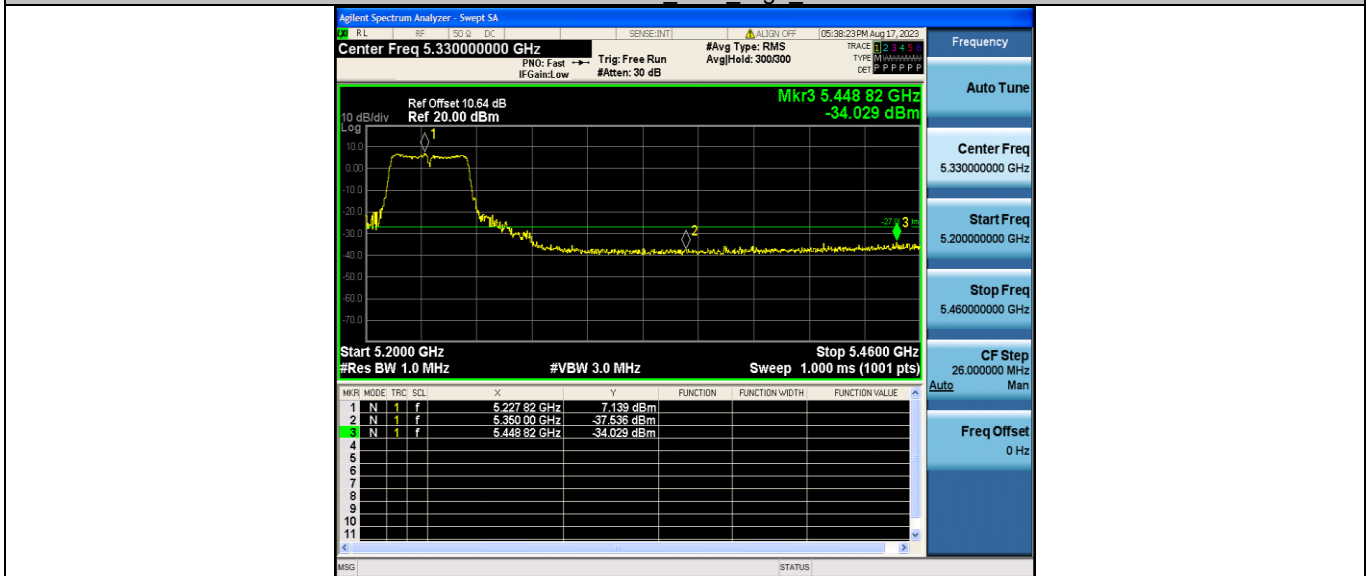
11AC40MIMO_Ant2_High_5230
