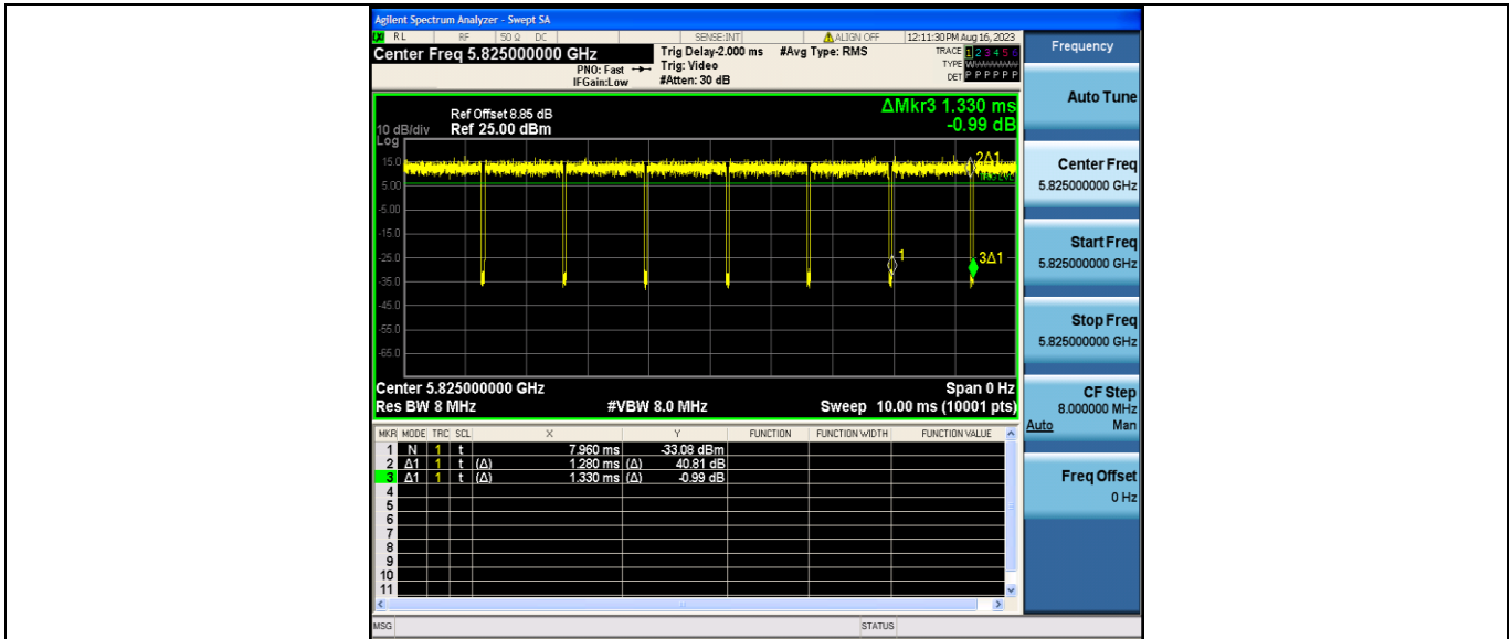
11AC20SISO_Ant2_5825
