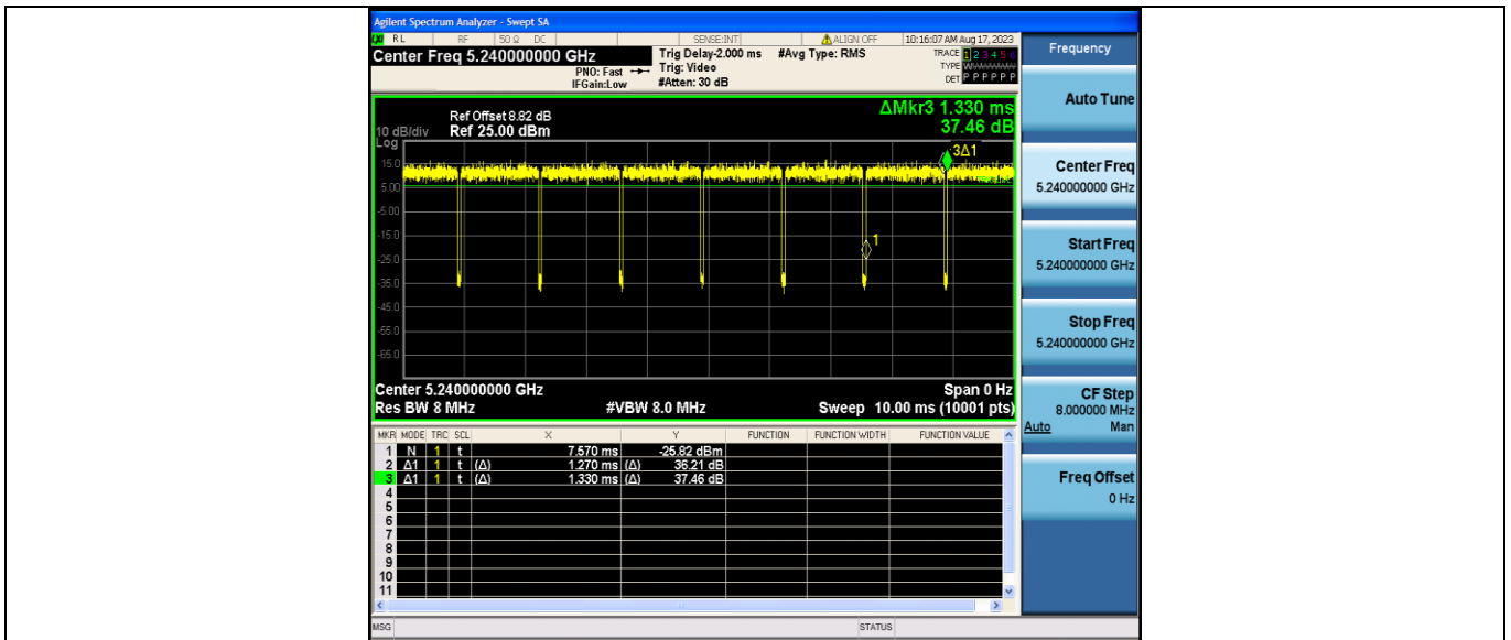
11N20MIMO Ant2 5240
