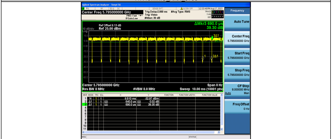
11N40MIMO Ant2 5795
