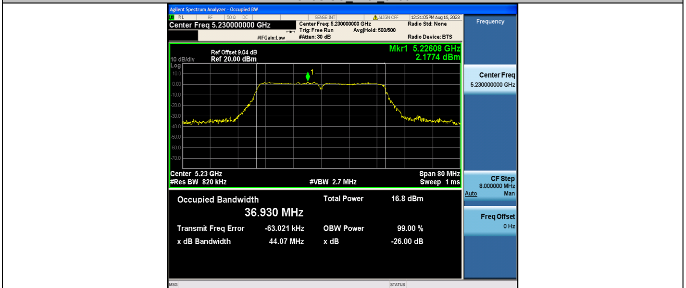
11AC40SISO_Ant2_5230
