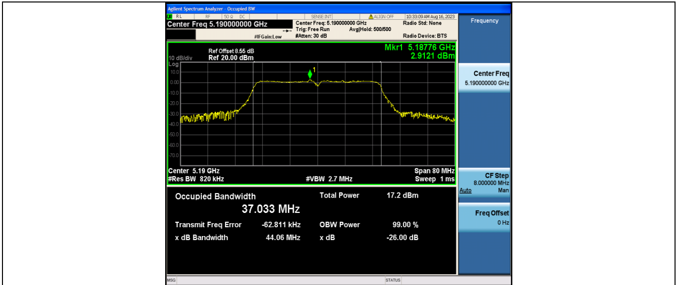
11N40SISO_Ant2_5190
