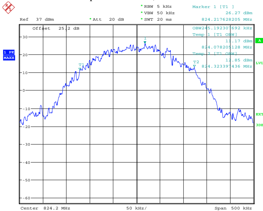
99% Occupied Bandwidth, Low Channel
