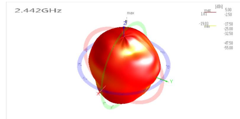
3D radiation pattern @2442MHz
