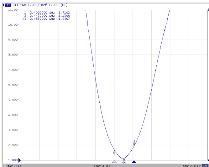
Return Loss & VSWR
