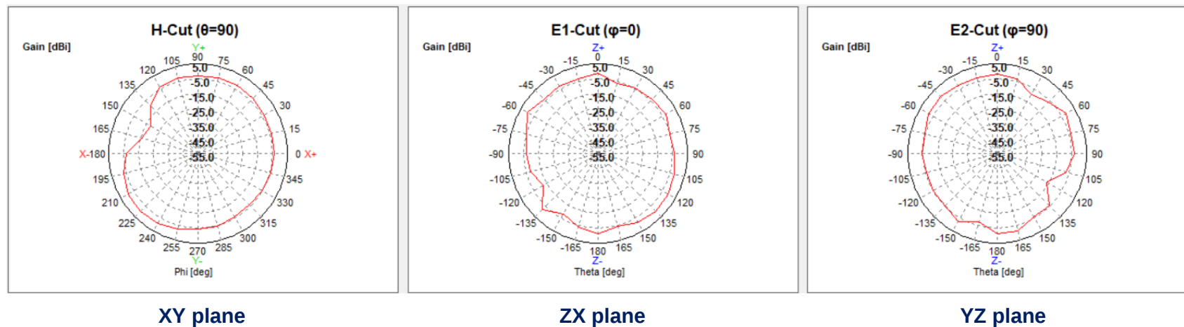
2D radiation pattern @2442MHz
