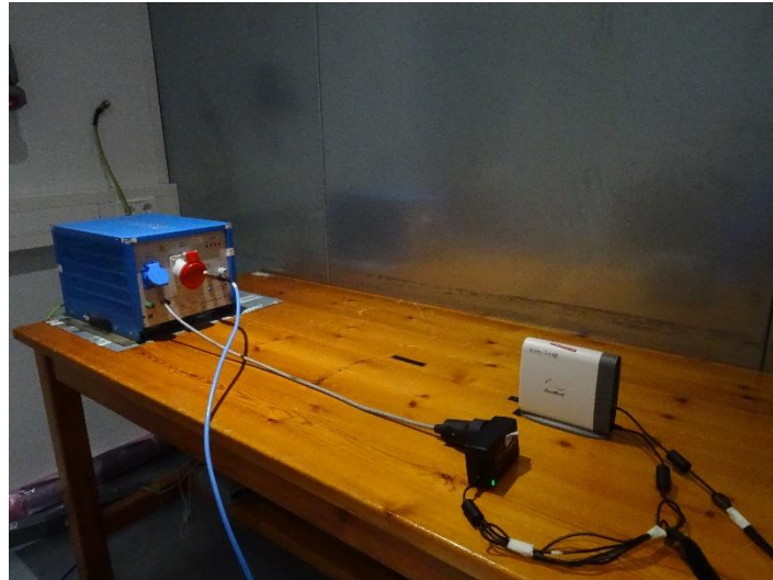
Conducted emission test for Sample S/01
