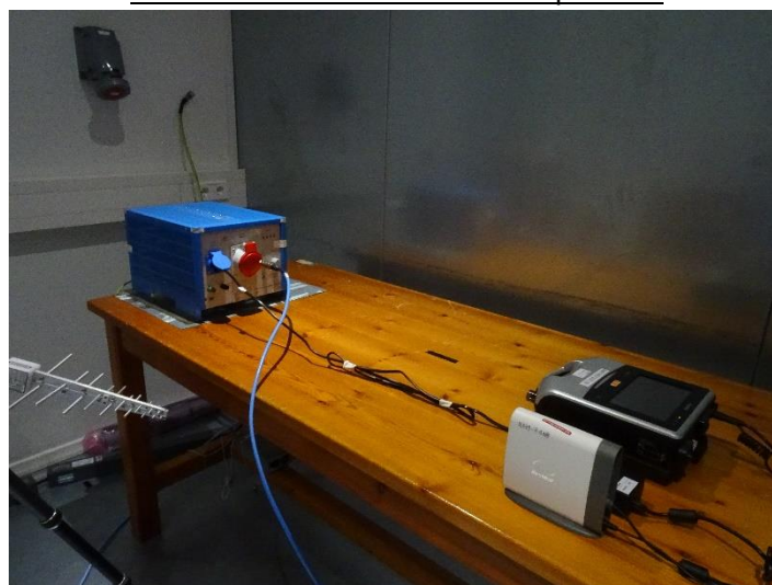
Conducted emission test for sample S/02
