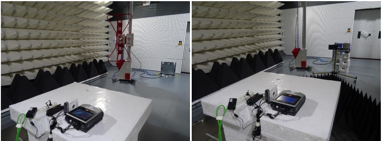
Radiated emission test for sample S/02
