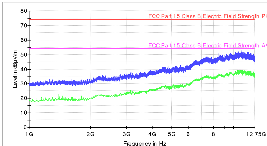
— Average Scan — Peak Scan — FCC Part 15 Class B Electric Field Strength PK — FCC Part 15 Class B Electric Field Strength AV
