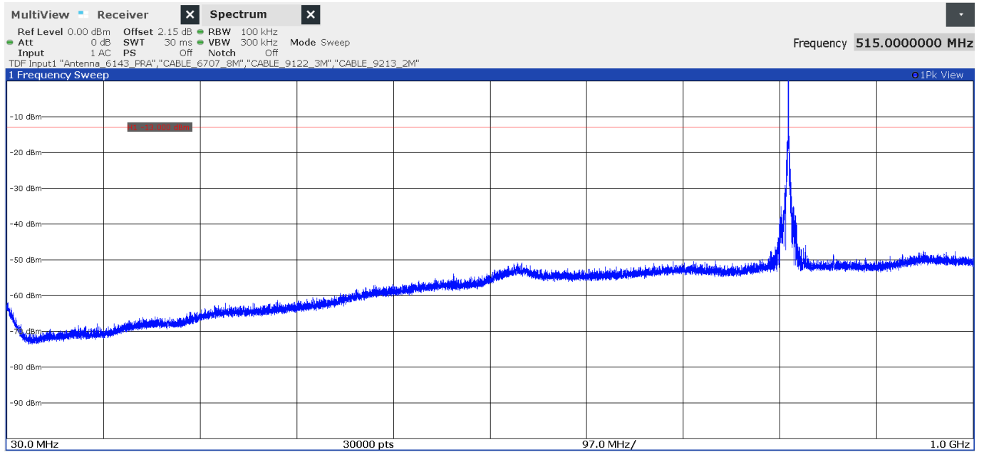
The peak above the limit is the carrier frequency: LTE Band 26, 814.7 MHz
