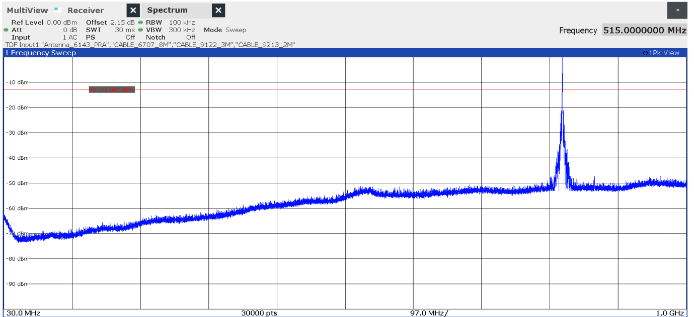
The peak above the limit is the carrier frequency: LTE Band 26, 824 MHz
