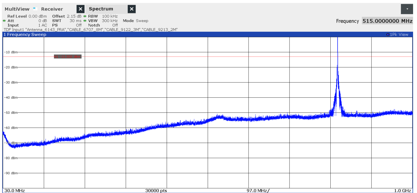
The peak above the limit is the carrier frequency: LTE Band 26, 819.3 MHz
