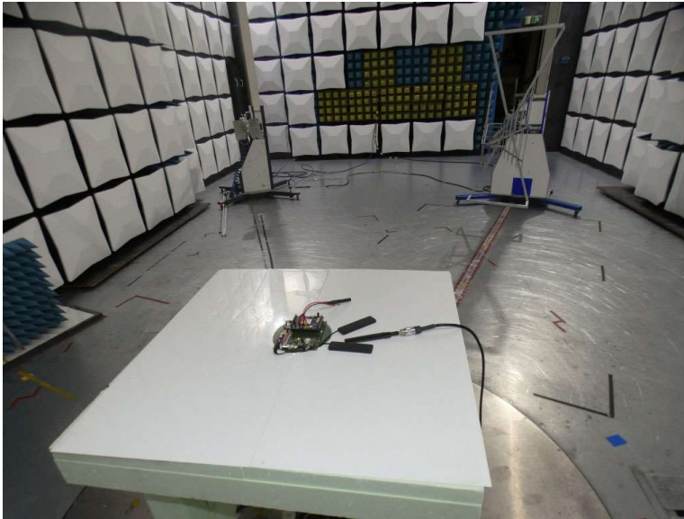
Photo 6: Test Antenna
