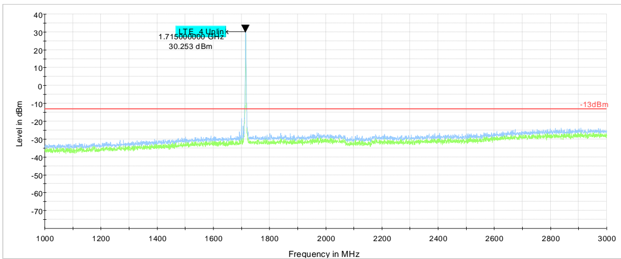
Plot # 44 Radiated Emissions: 1 GHz - 3 GHz
