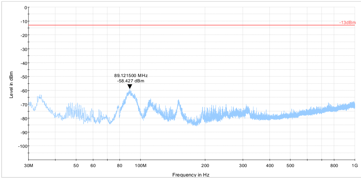
Plot # 12 Radiated Emissions: 30 MHz - 1 GHz
