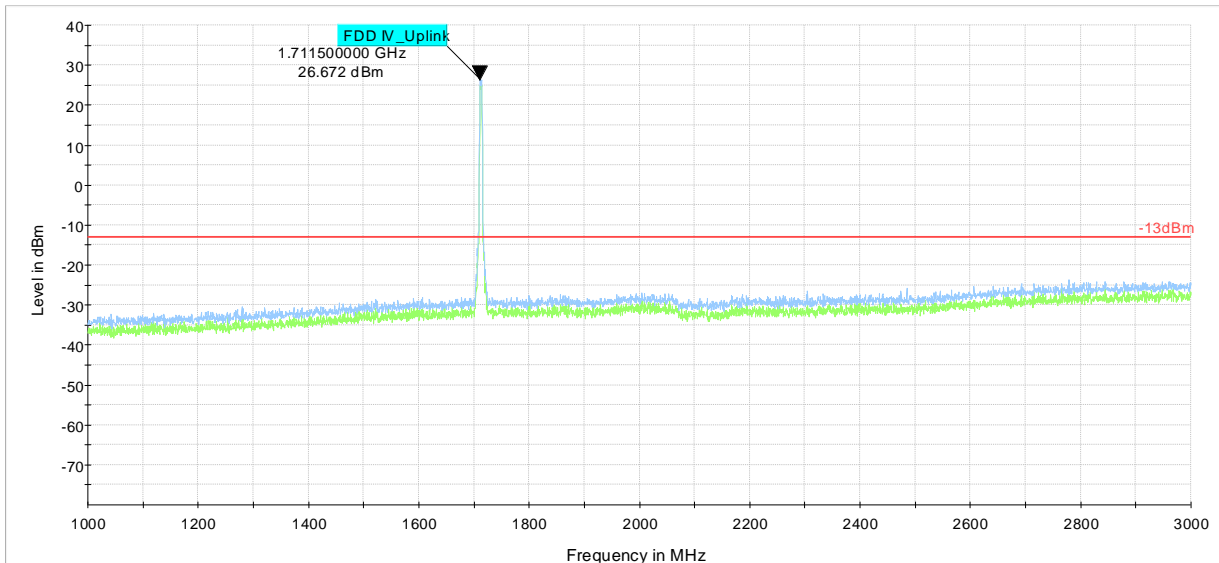
Plot # 13 Radiated Emissions: 1 GHz - 3 GHz
