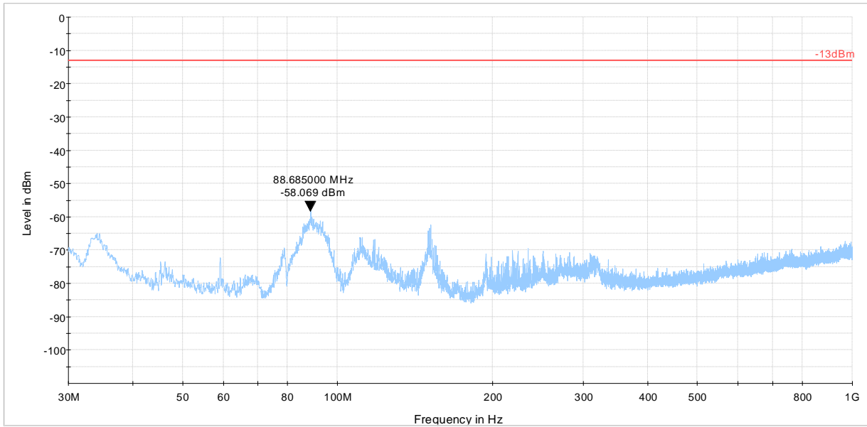
Plot # 43 Radiated Emissions: 30 MHz - 1 GHz
