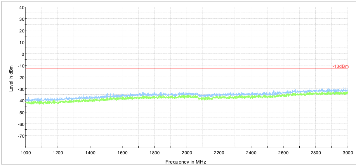
Plot # 23 Radiated Emissions: 1 GHz - 3 GHz
