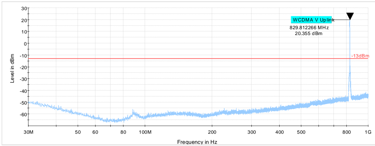
Plot # 22 Radiated Emissions: 30 MHz - 1 GHz
