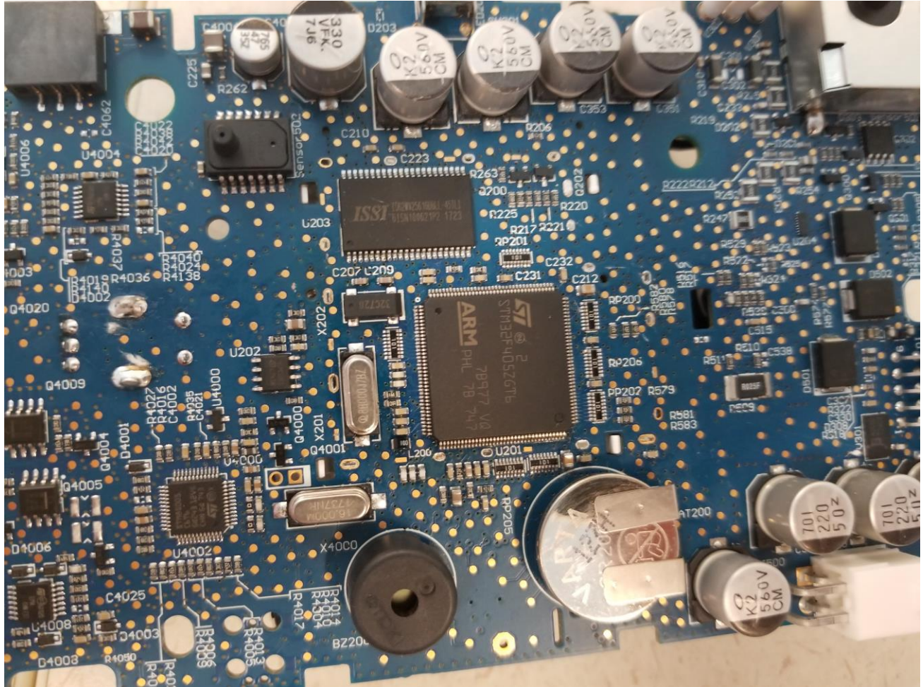
Back of Flow Generator Mother Board without Processor Shield Can
