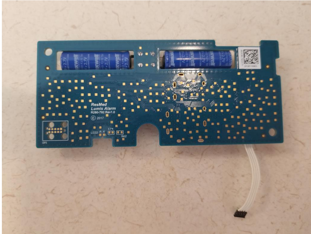
Top Side of Alarm Board
