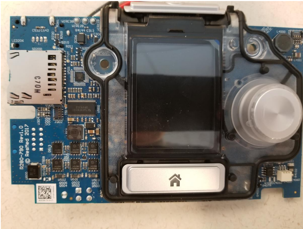
Display Side of Flow Generator Mother Board
