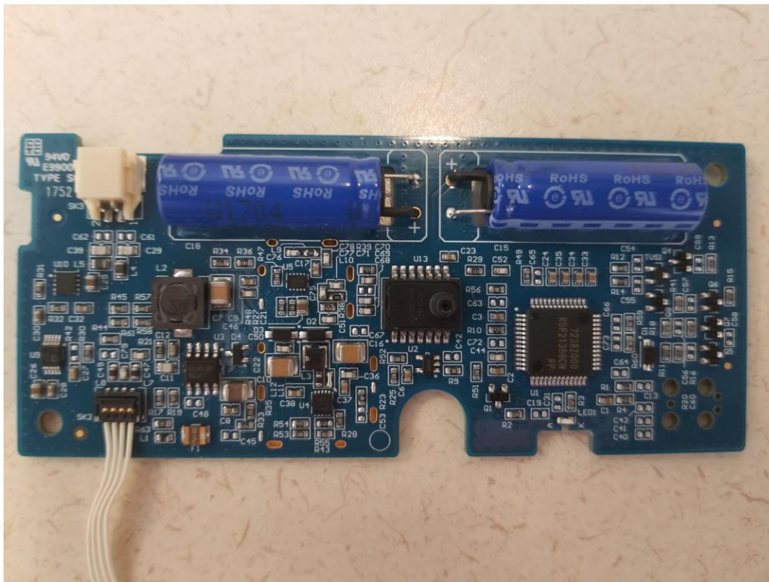
Bottom side of Alarm Board
