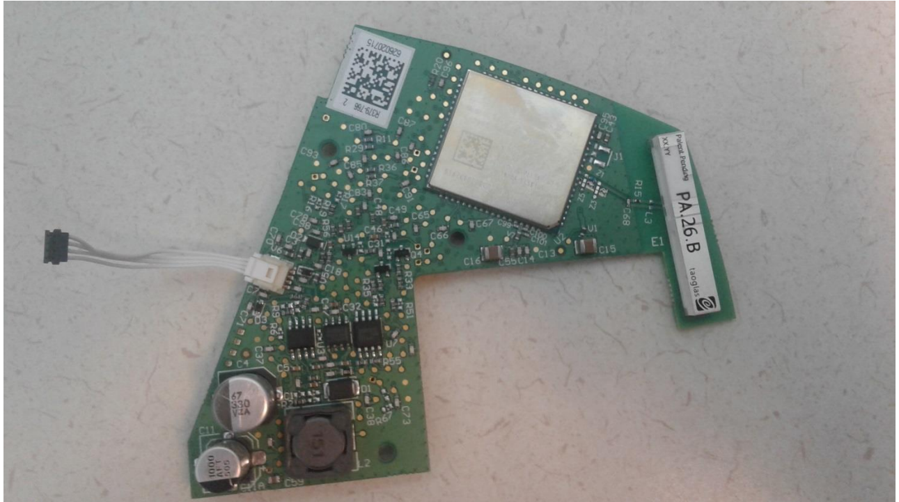
Cellular Module & Antenna Side of CAM_Board
